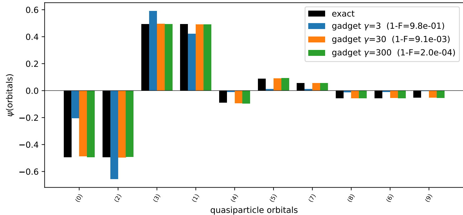
Ca42 - particle conservation (10 qubits)
