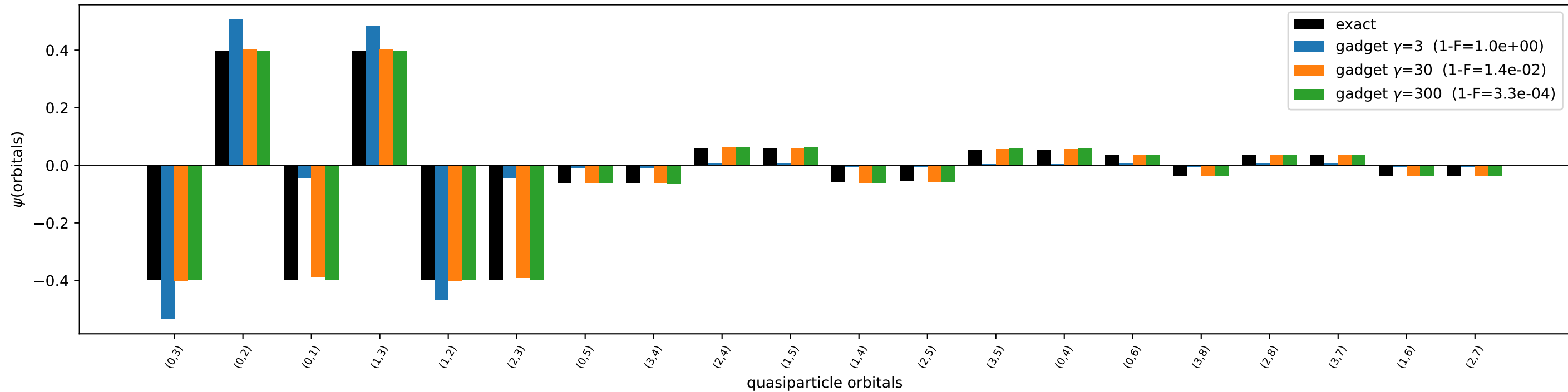
Ca44 - first quantization (20 qubits, top 20/45)
