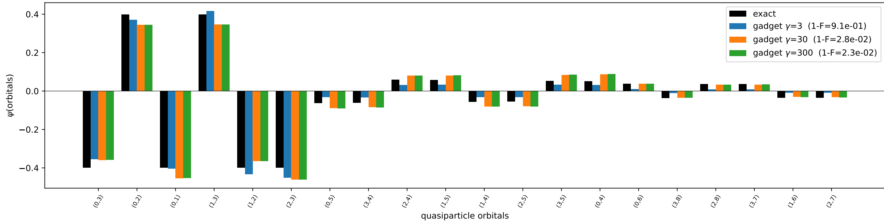
Ca44 - particle conservation (10 qubits, top 20/45)
