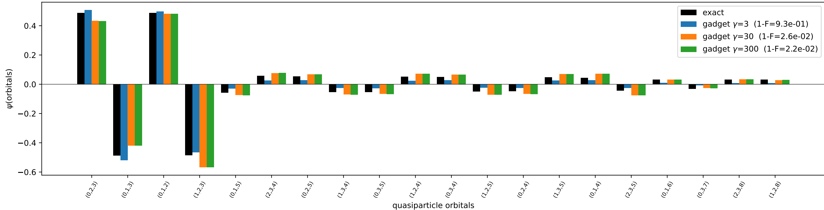
Ca46 - particle conservation (10 qubits, top 20/120)
