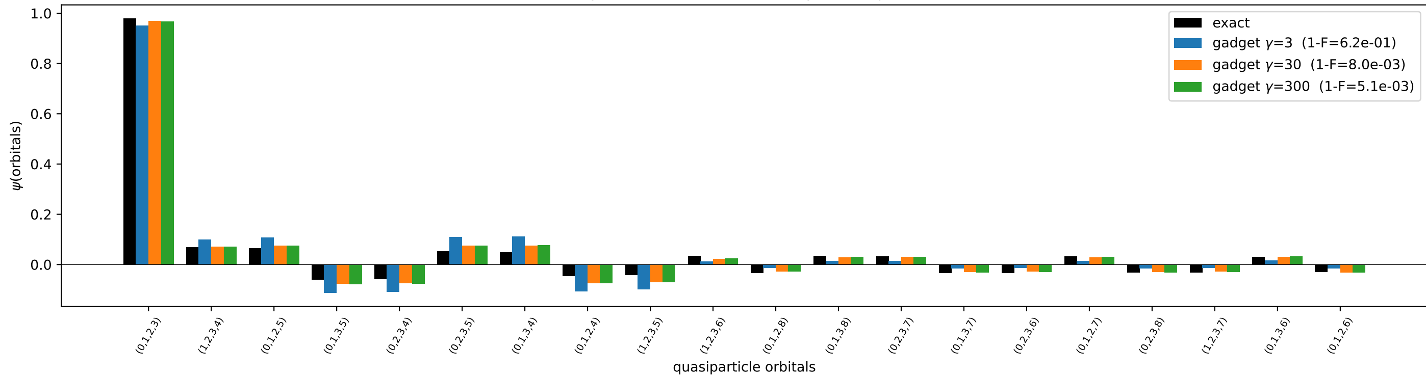
Ca48 - particle conservation (10 qubits, top 20/210)
