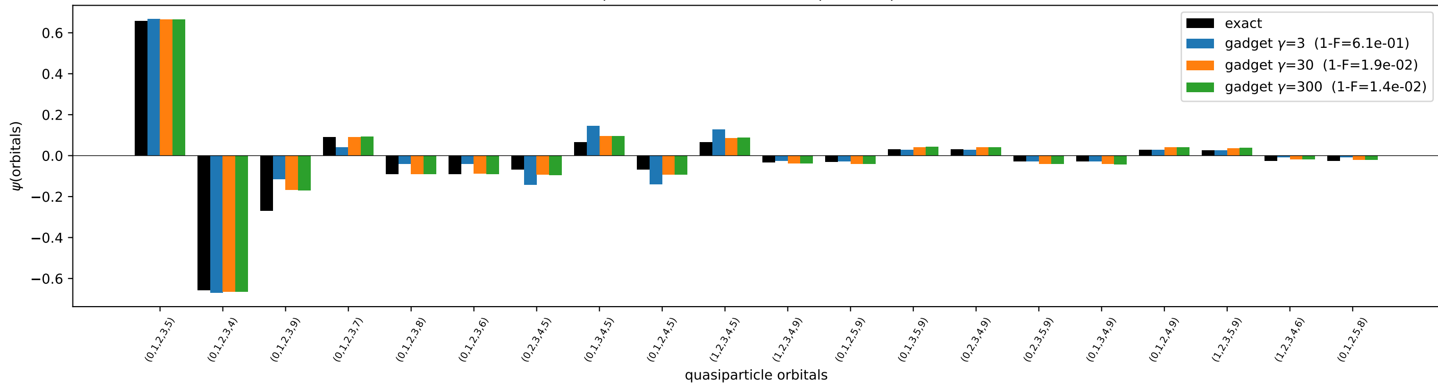
Ca50 - particle conservation (10 qubits, top 20/252)
