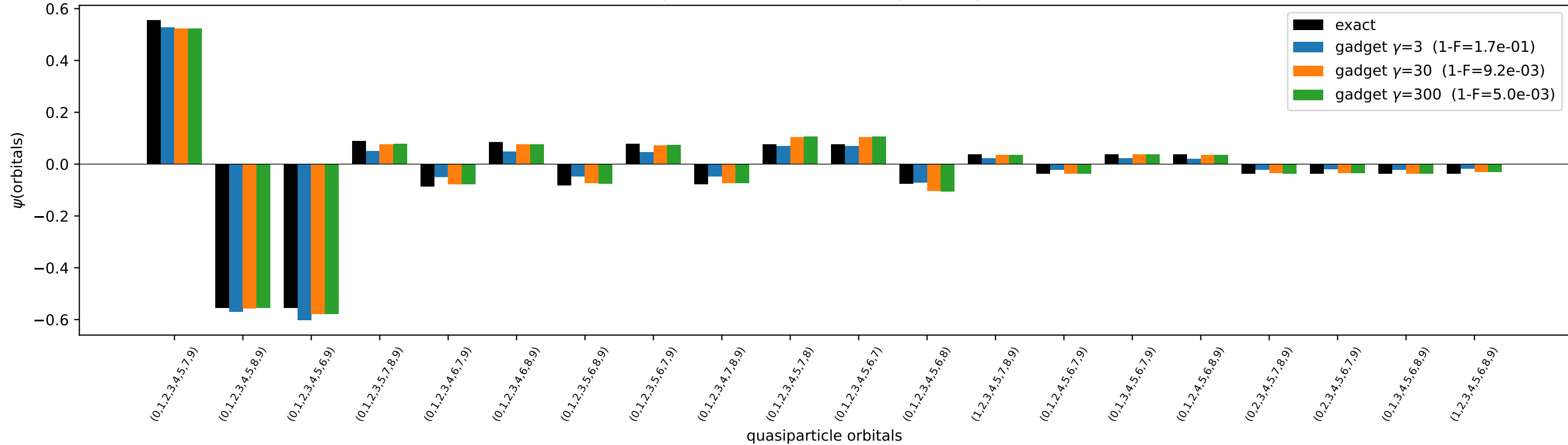
Ca56 - particle conservation (10 qubits, top 20/45)
