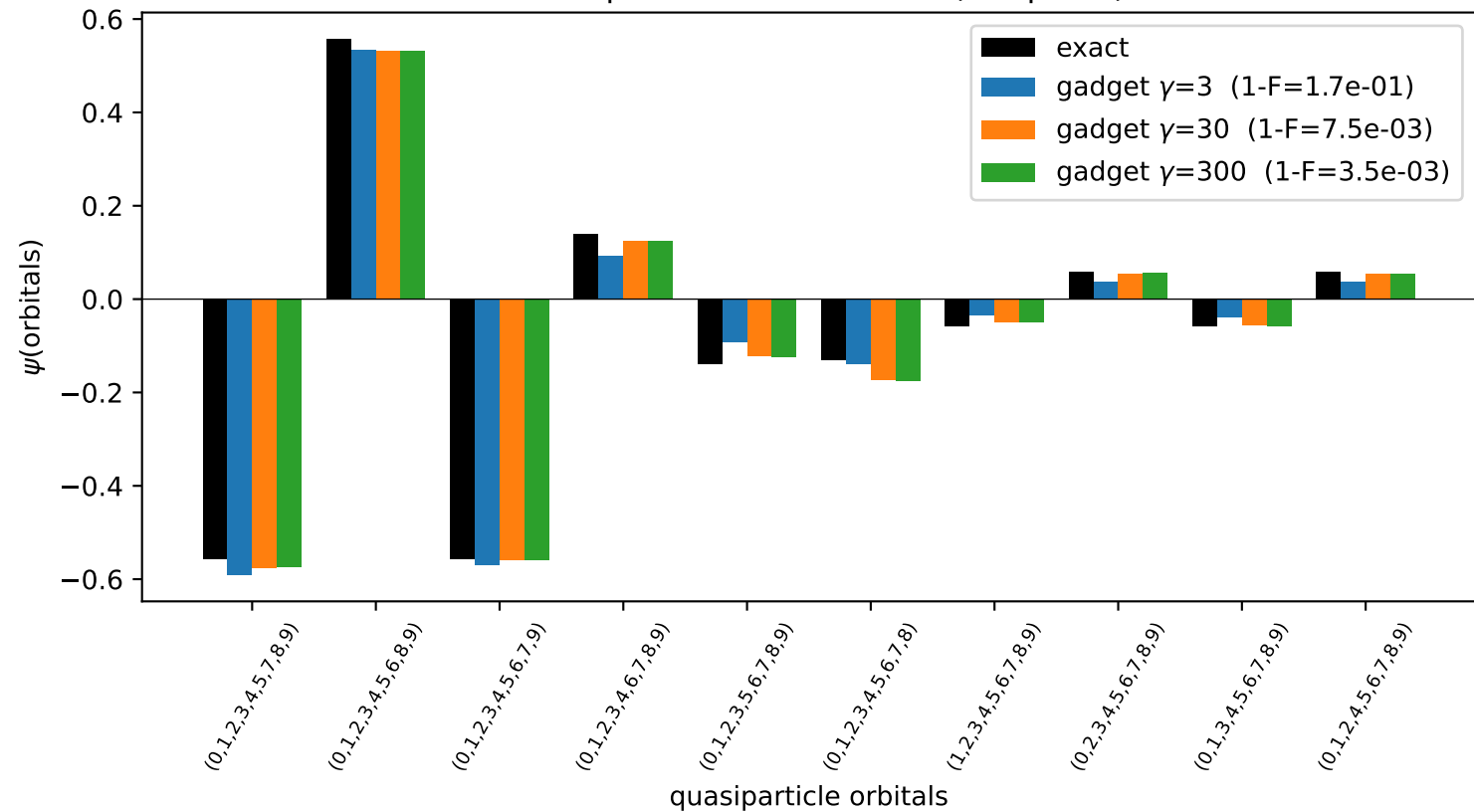
Ca58 - particle conservation (10 qubits)
