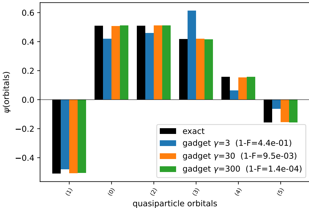
O18 - first quantization (6 qubits)
