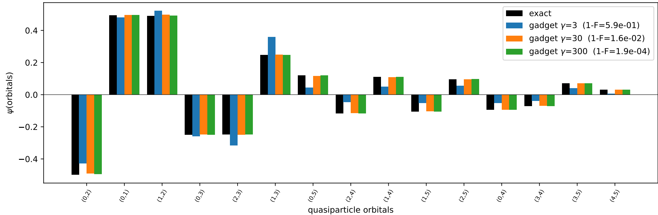
O20 - first quantization (12 qubits)
