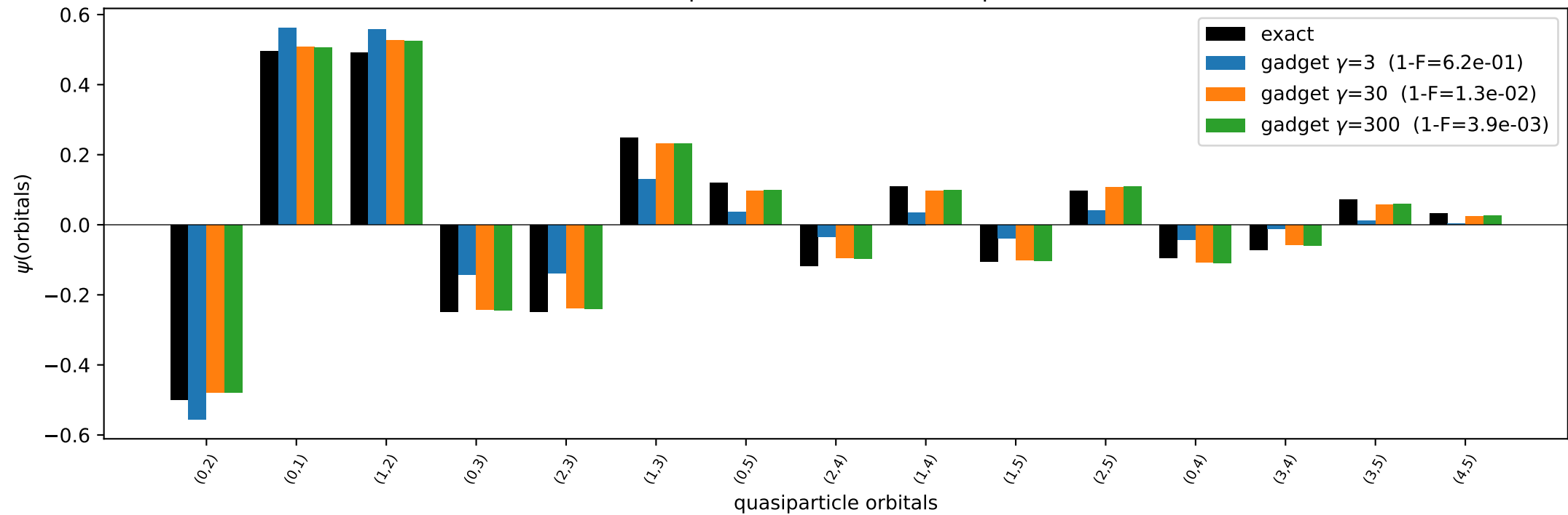
O20 - particle conservation (6 qubits)
