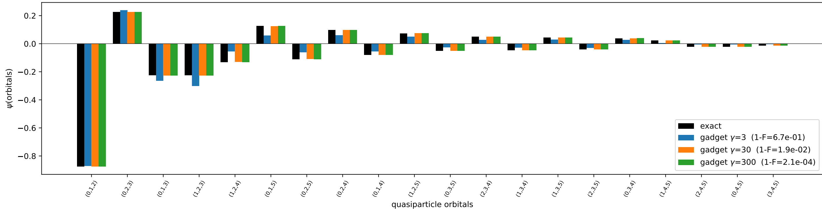
O22 - first quantization (18 qubits)
