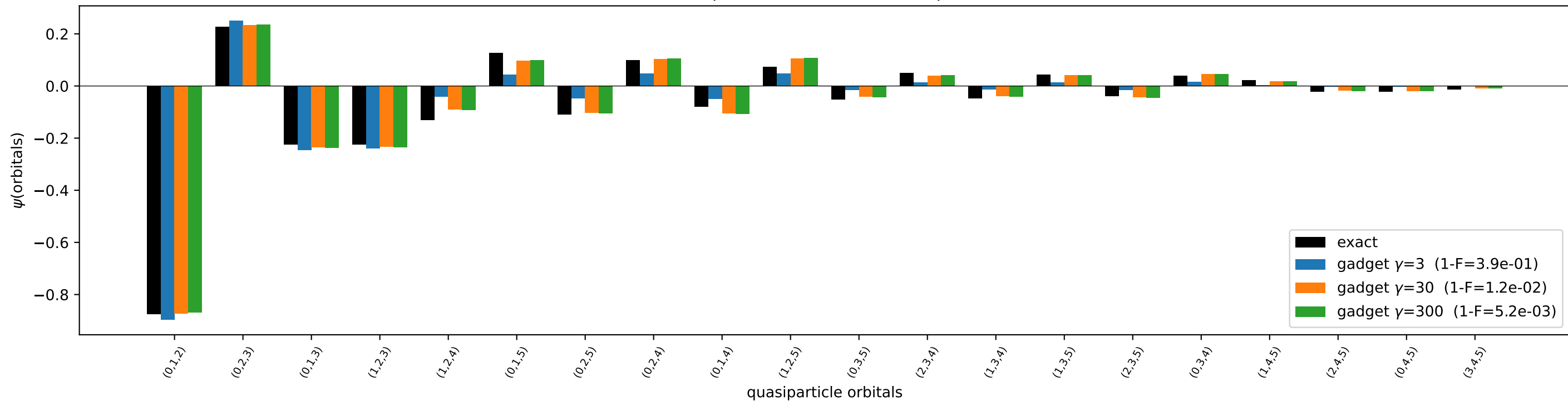
O22 - particle conservation (6 qubits)
