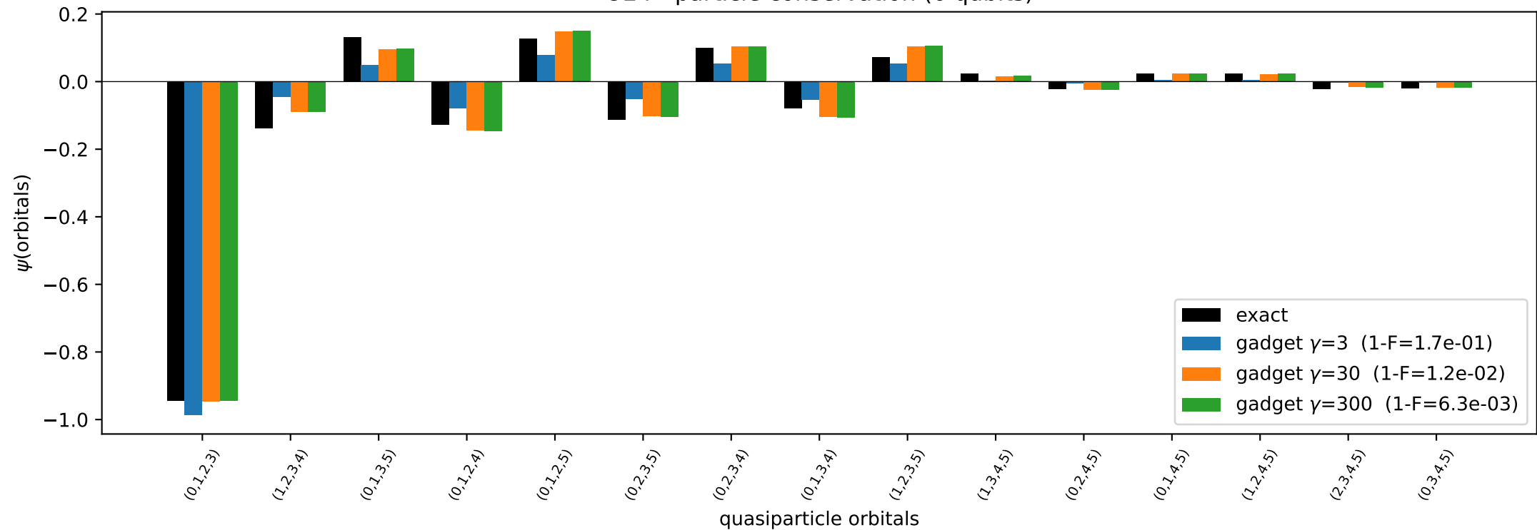
O24 - particle conservation (6 qubits)
