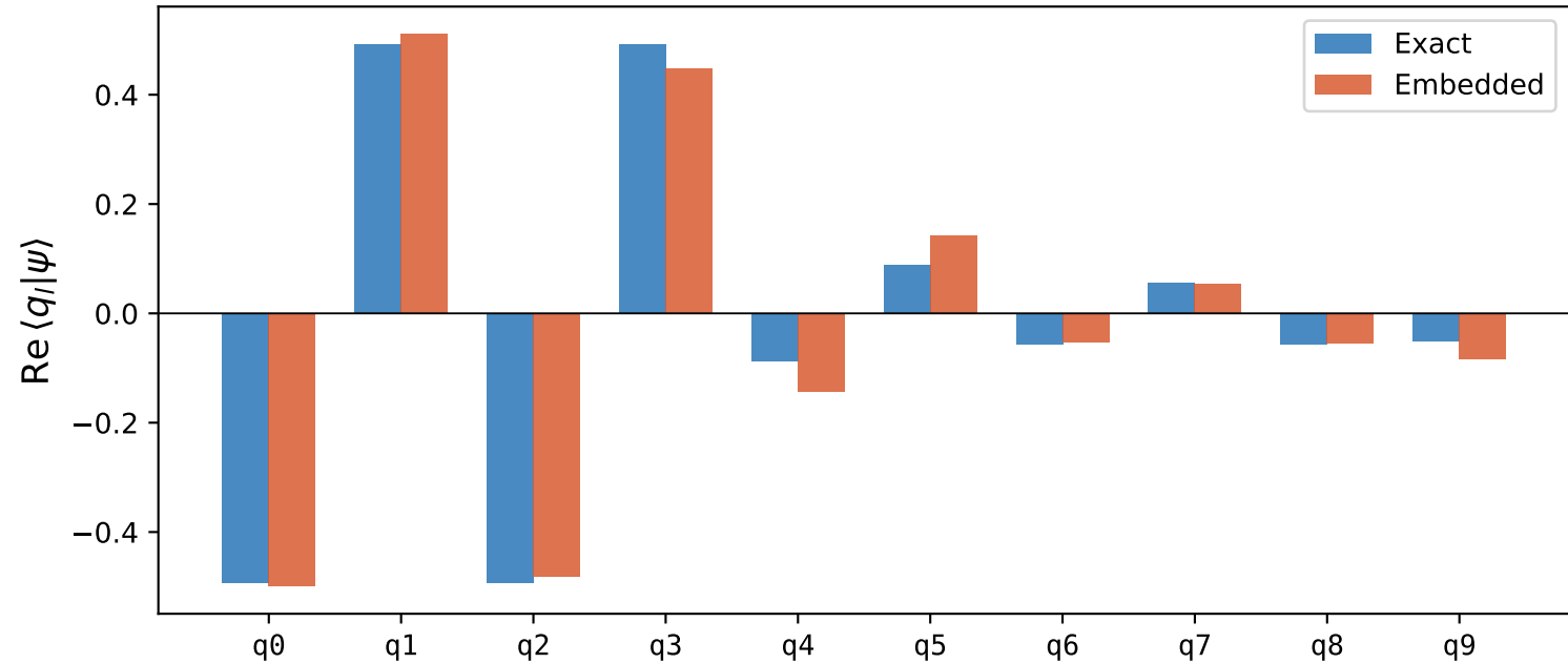
Real part of amplitudes — N=1 sector \gamma=100 , J_F=1000 , Fidelity=0.98888
