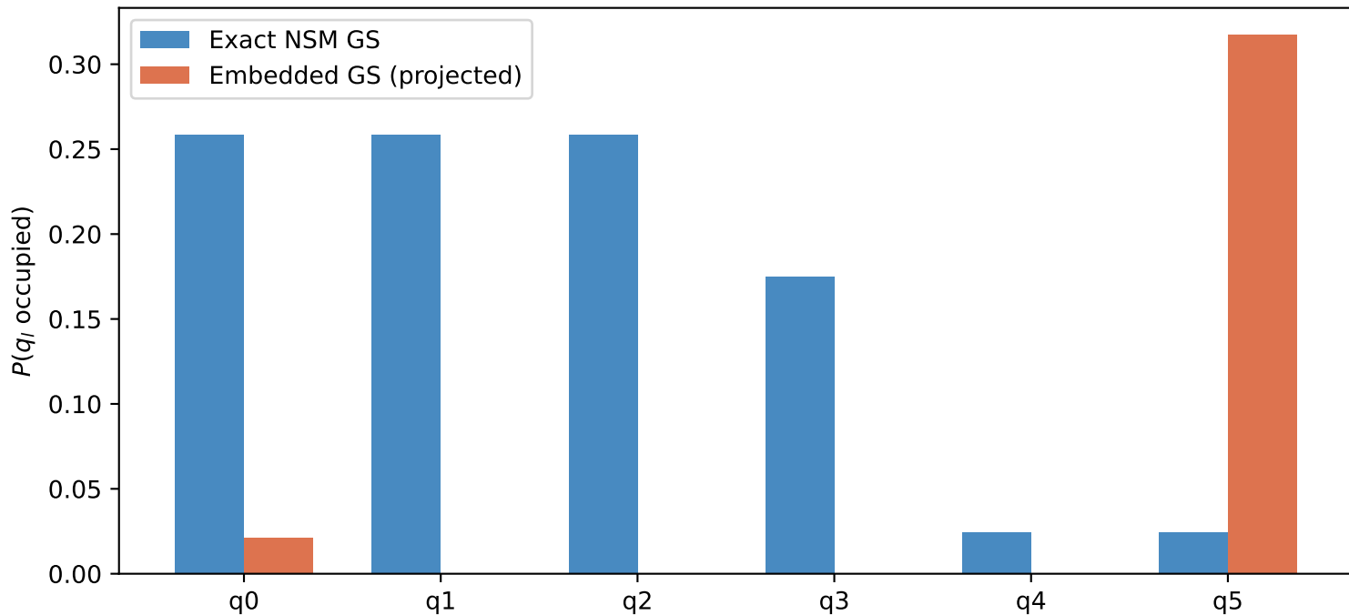
Exact vs. Embedded Ground State — Logical Qubit Occupancies
