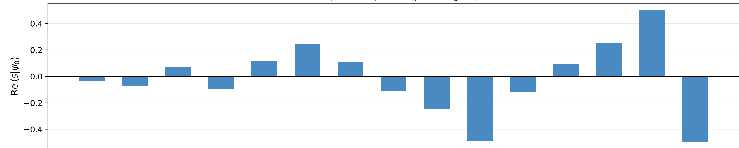
Real part of amplitudes (phase-aligned)
