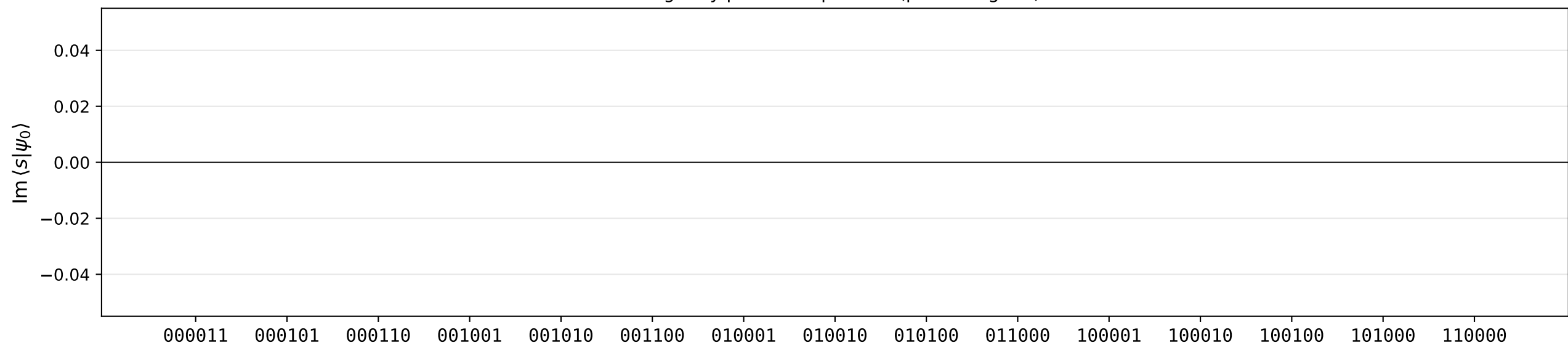
Imaginary part of amplitudes (phase-aligned)
