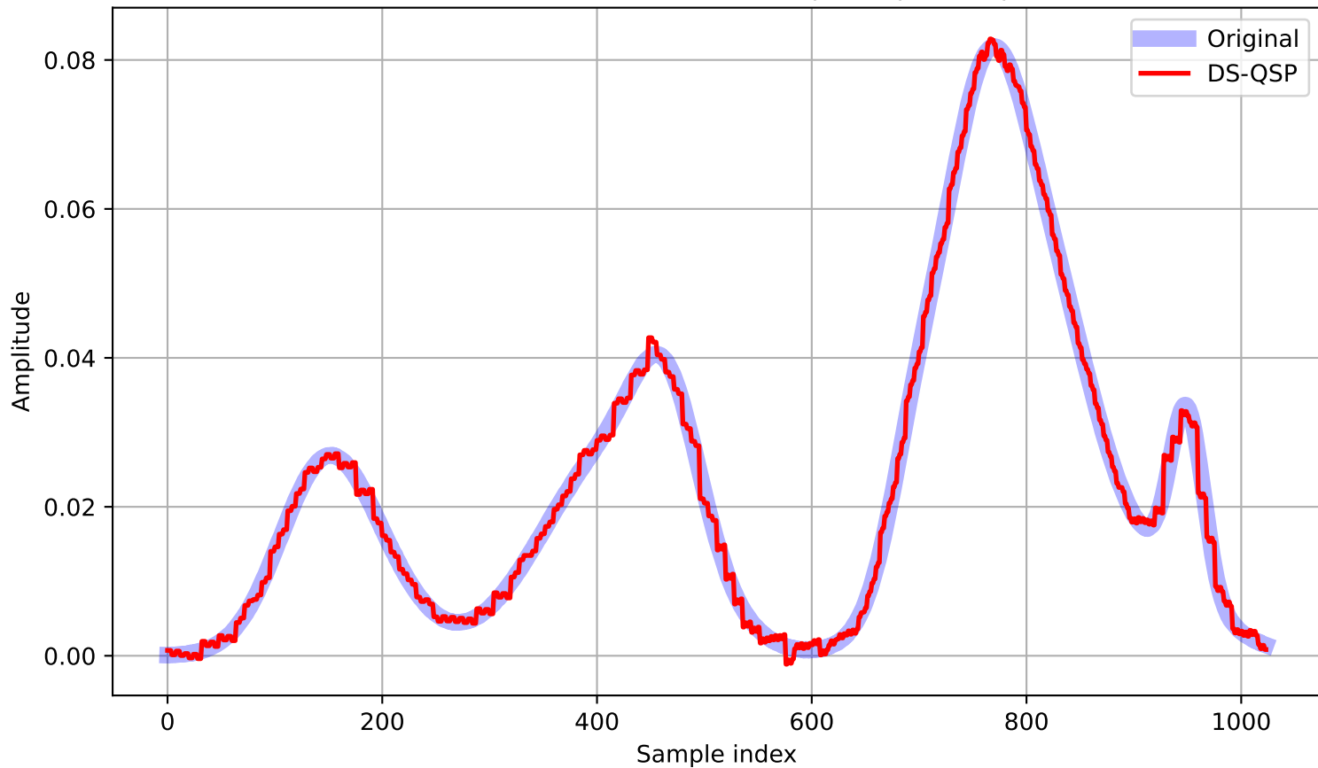
Lossy DS-QSP: Mixture of Gaussian Signal | L=9 | k=65 | TD = 3.18e-02
