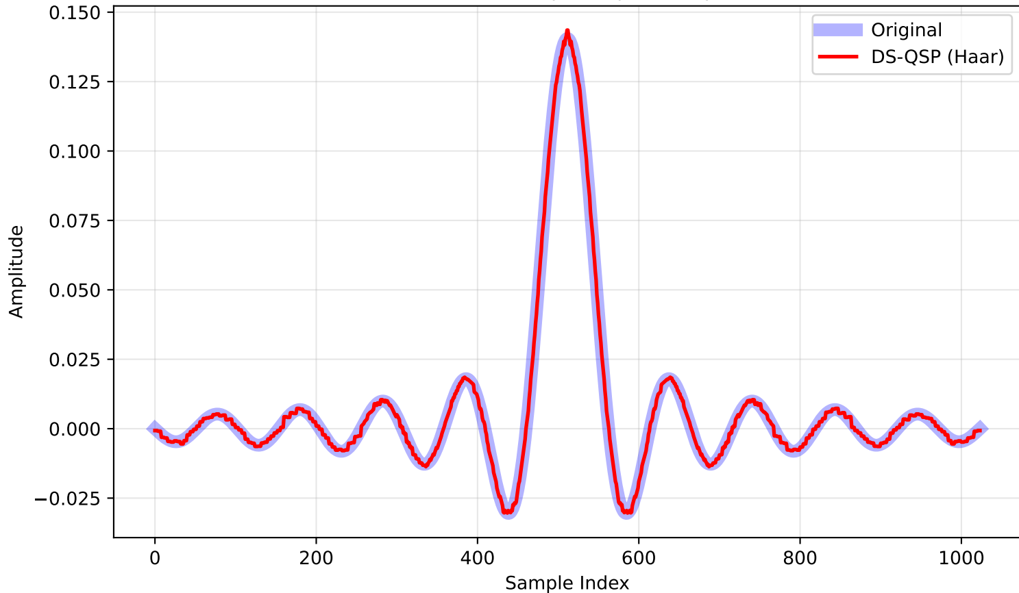
Lossy DS-QSP: Sinc Signal | L=8 | k=136 | TD = 1.94e-02
