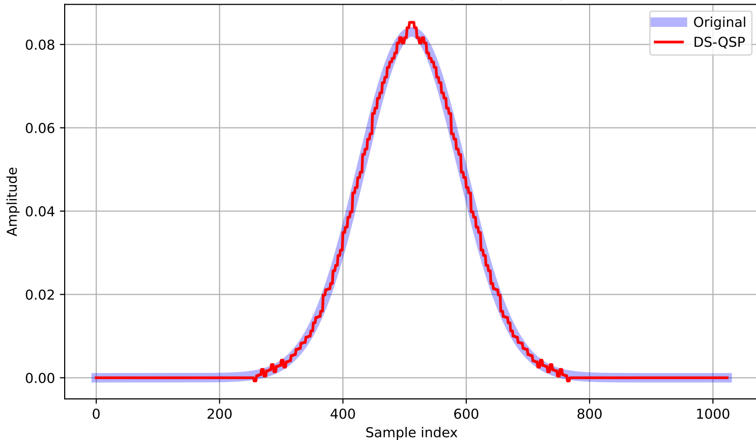
Lossy DS-QSP: Single Gaussian Signal | L=8 | k=30 | TD = 2.04e-02
