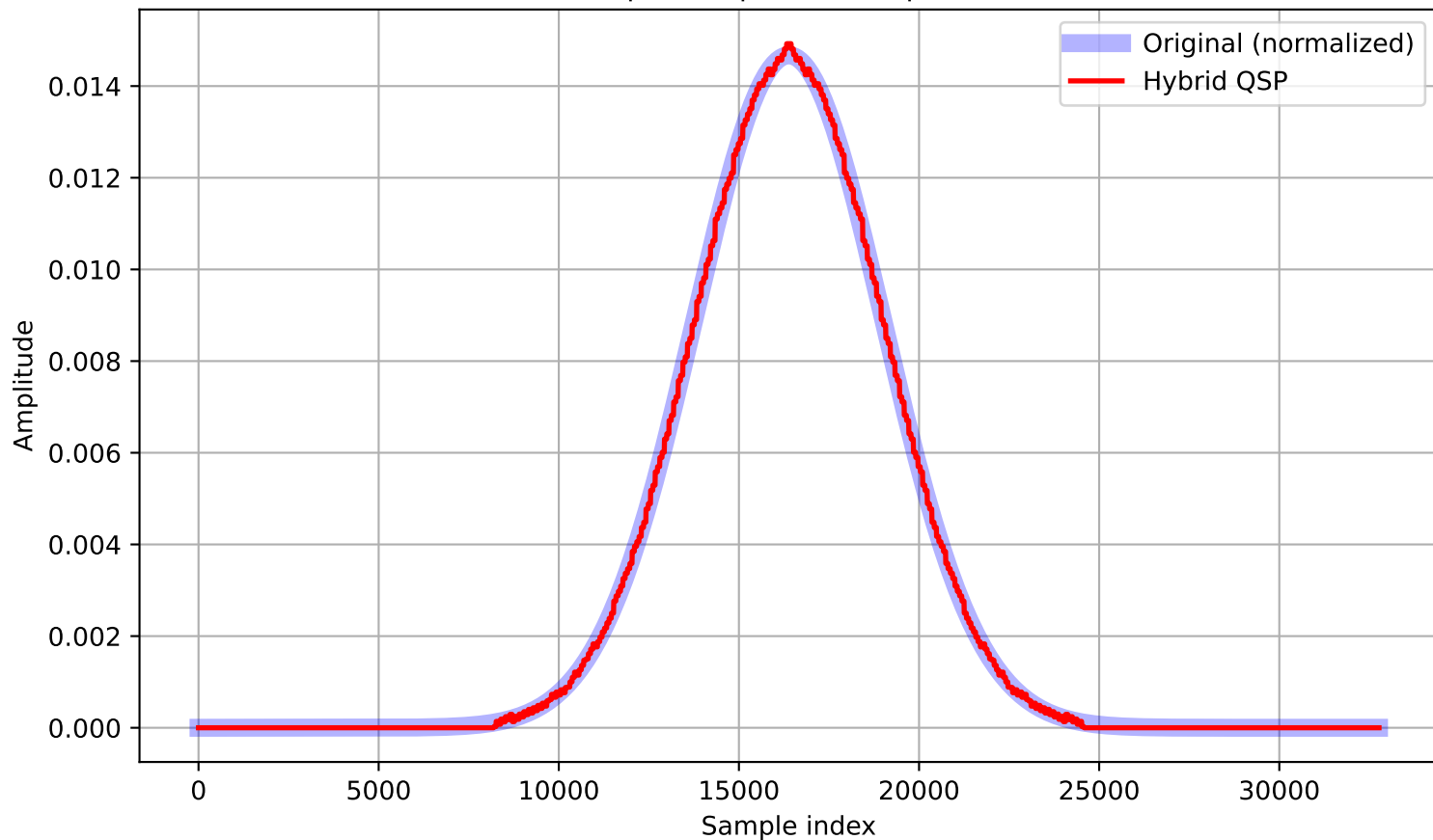
Sinc-Gaussian | L=13 | thr-k=44 | TD=1.0194e-02
