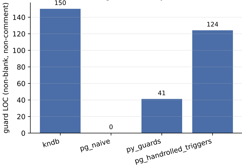
Lines of guard code by baseline
