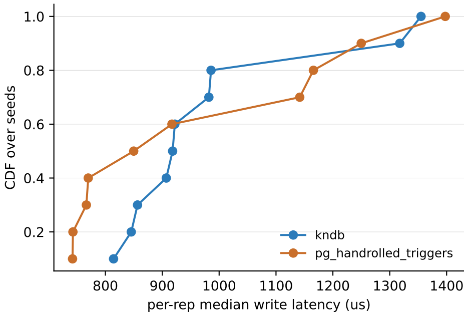
Write-latency CDF (10k rows/rep, seed reps)
