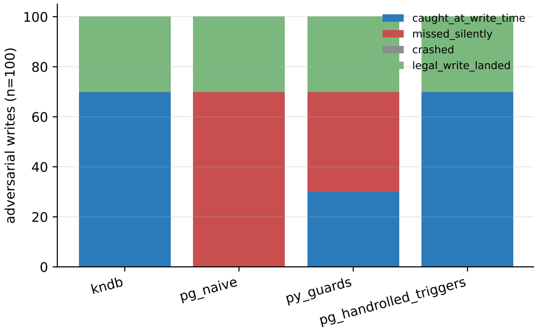
Adversarial write outcomes per system
