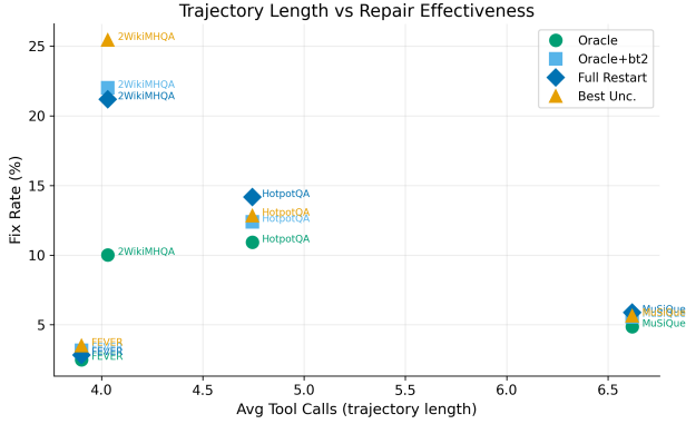
Figure 5: Trajectory length vs. repair effectiveness. Shorter trajectories (FEVER, 2WikiMHQA) favor targeted repair; longer trajectories (HotpotQA, MuSiQue) favor full restart, consistent with the context contamination hypothesis.
