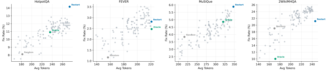
Figure 4: Cost-accuracy Pareto fronts for all four datasets. Each grey dot is an individual repair strategy; labeled points show baselines. On 2WikiMultiHopQA, many uncertainty strategies dominate the Pareto front above Full Restart.
