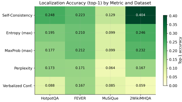
Figure 3: Localization accuracy (argmax top-1) by uncertainty metric and dataset. Self-consistency achieves the highest accuracy across all benchmarks, reaching 0.404 on 2WikiMultiHopQA.
