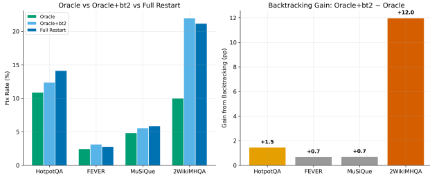
Figure 2: Left: Oracle, Oracle+bt2, and Full Restart fix rates. Right: Backtracking gain (Oracle+bt2 – Oracle). The +12.0 pp gain on 2WikiMultiHopQA confirms strong error cascade effects.
