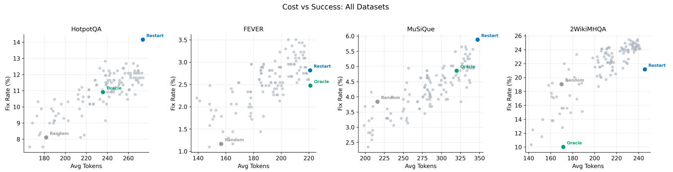
Figure 5: Cost-accuracy Pareto fronts for all four datasets. Each grey dot is an individual repair strategy; labeled points show baselines. On 2WikiMultiHopQA, many uncertainty strategies dominate the Pareto front above Full Restart.
