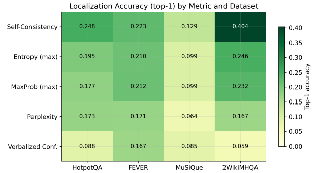
Figure 3: Localization accuracy (argmax top-1) by uncertainty metric and dataset. Self-consistency achieves the highest accuracy across all benchmarks, reaching 0.404 on 2WikiMultiHopQA.
