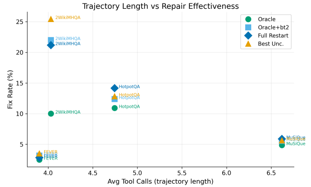
Figure 4: Trajectory length vs. repair effectiveness. Shorter trajectories (FEVER, 2WikiMHQA) favor targeted repair; longer trajectories (HotpotQA, MuSiQue) favor full restart, consistent with the context contamination hypothesis.
