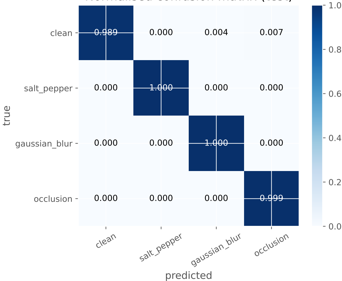
Normalised confusion matrix (test)
