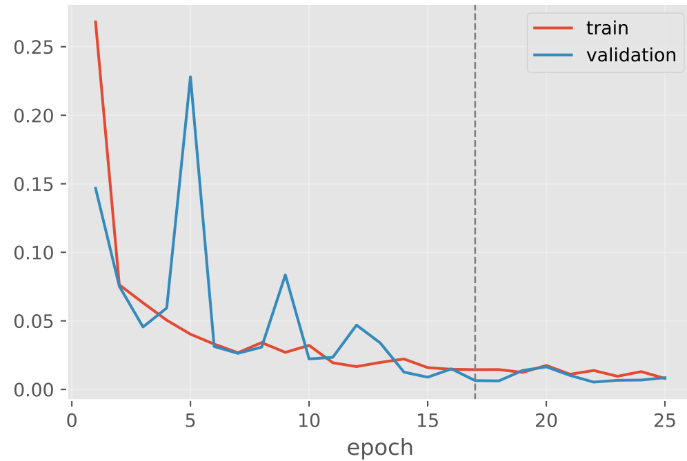
Cross-entropy
