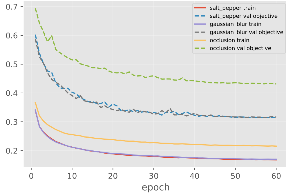
Loss
