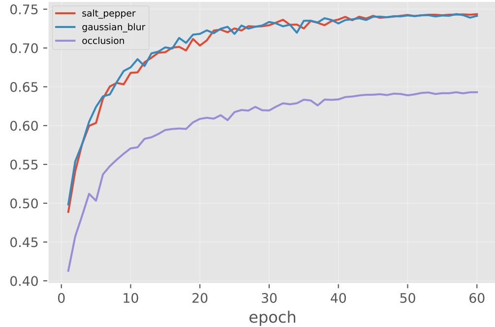
Validation SSIM
