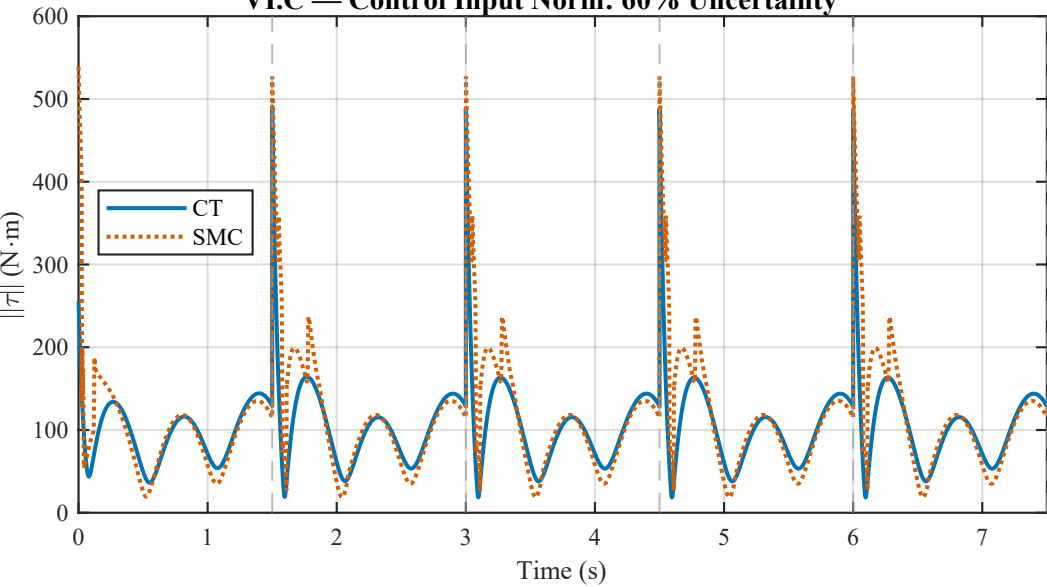
VI.C — Control Input Norm: 60% Uncertainty
