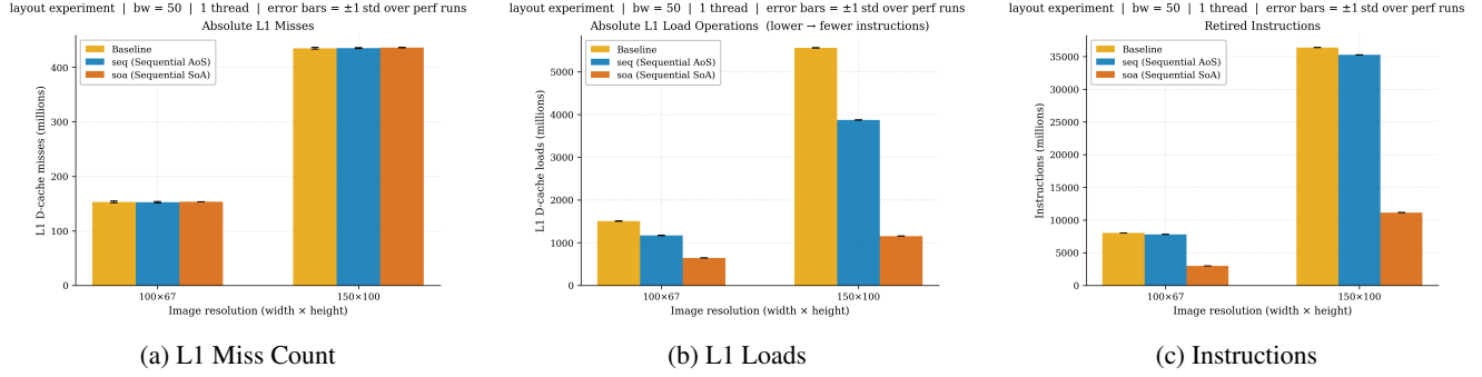
Figure 4: Comprehensive profile metrics including L1 cache misses, total loads, and instruction counts.
