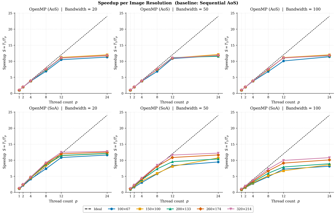
Figure 6: The near-linear scaling at 12 cores ( \approx 11\times ) confirms efficient parallelization, while SMT (24 threads) provides marginal additional benefit ( \approx 11.5\times ).
