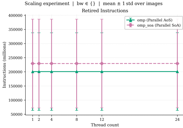
Figure 8: Total instructions per iteration for omp and omp_soA across thread counts. The count is flat across all threads (OpenMP adds zero overhead); SoA executes \sim 14\% more instructions due to its five-stream memory layout.
