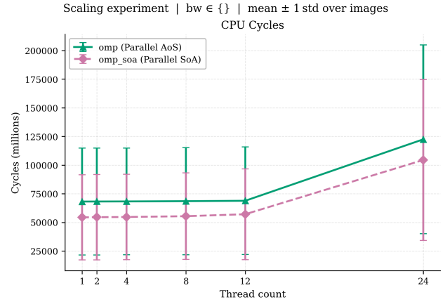
Figure 10: Total CPU cycles per iteration. Cycles are flat up to 12 physical cores (zero parallel overhead), then approximately double at 24 threads under SMT contention. The jump is similar for both variants, confirming a hardware-level effect.
