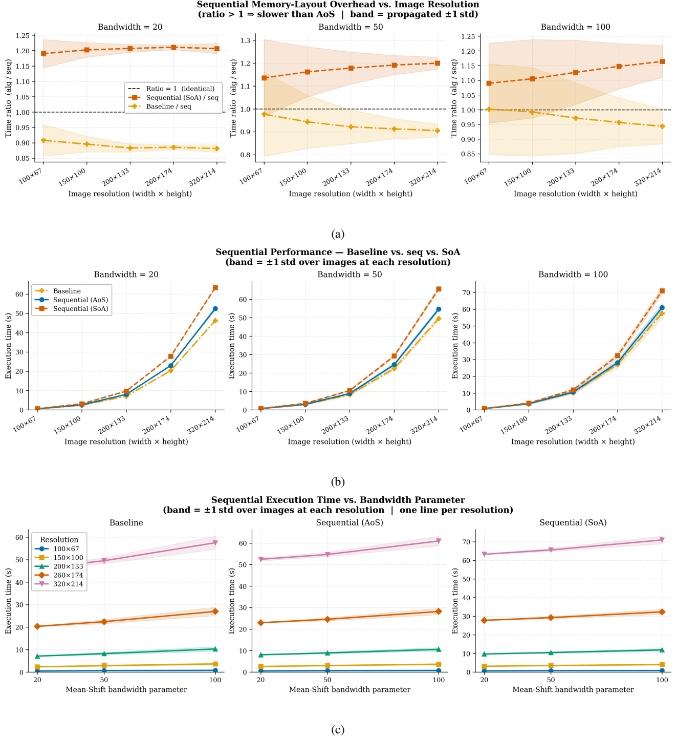
Figure 7: Sequential performance profiling of Mean Shift variants utilizing a dynamically swappable kernel on the AMD Ryzen 9900X. The abstraction overhead of this kernel design fundamentally inhibits compiler auto-vectorization. The resulting absence of SIMD acceleration dictates the anomalous performance characteristics observed across all three subfigures. (a) Memory layout overhead. The naive Baseline unexpectedly outperforms both pre-computed AoS and SoA layouts. Without SIMD registers to rapidly consume contiguous data, the memory-bound optimizations of SoA introduce detrimental scalar load latency. (b) Execution latency scaling. The Baseline maintains superior performance across spatial resolutions. In a purely scalar execution regime, the overhead of fetching disparate pre-computed coordinates from the L1 cache exceeds the latency of the Baseline’s on-the-fly arithmetic recomputation. (c) Bandwidth dependency. Expanding the spatial bandwidth introduces a distinct latency penalty. Lacking SIMD units to efficiently parallelize the \mathcal{O}(N^2) neighbor evaluations, the pipeline becomes saturated by compute-bound scalar operations, exposing the direct arithmetic cost of the expanded search volume.
