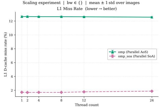
Figure 9: L1 data cache miss rate across thread counts. The SoA layout maintains \sim 1.7\% vs \sim 12.6\% for AoS at all thread counts, confirming the cache advantage is thread-count independent. Mild degradation at 24T (1.85%) suggests SMT cache-line bouncing.
