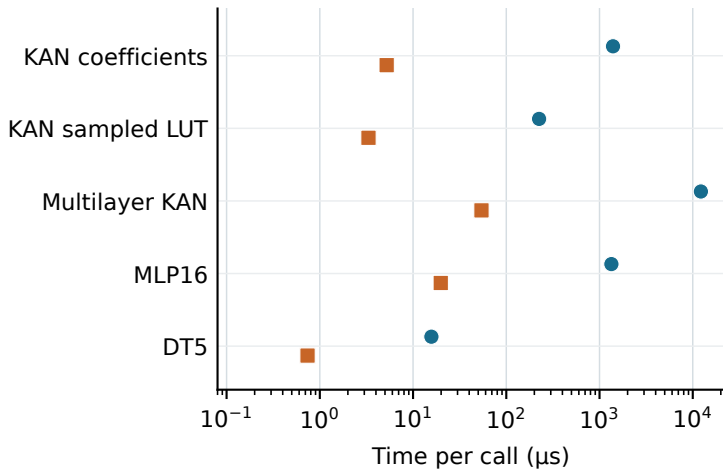
(a) Active batch timing
