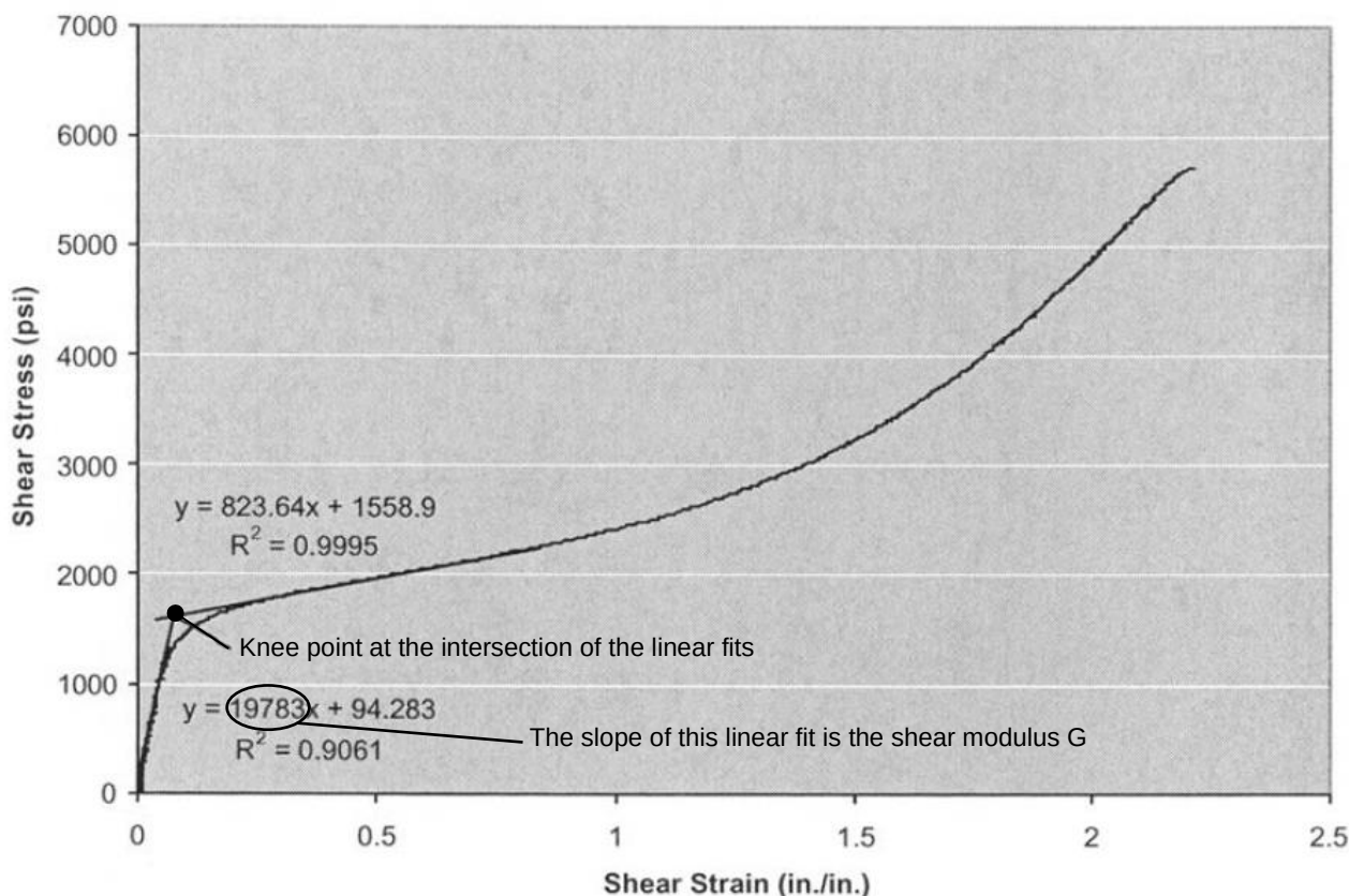
Figure 1. Example of shear stress-strain curve as defined per ASTM D5656 test method
