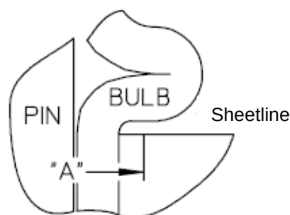
Figure 3- Gap between bulb-structure reaching fastener's shank – Not acceptable
