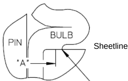
Figure 2- Abrupt change – Not acceptable bulb formation
