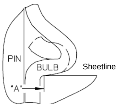
Figure 1- Acceptable bulb formation
