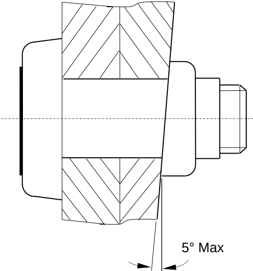
Maximum back side slope angle
