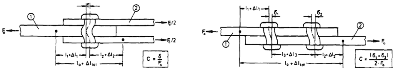
Figure 2. Double Shear and Single Shear configurations
