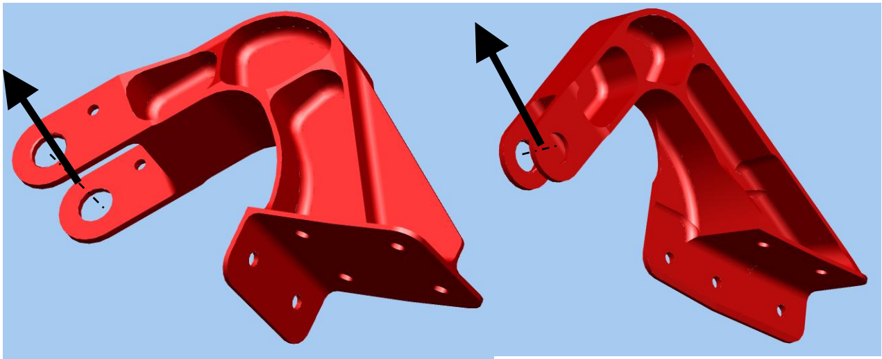
Figure 11. Fitting with non-plane bolted attachment
