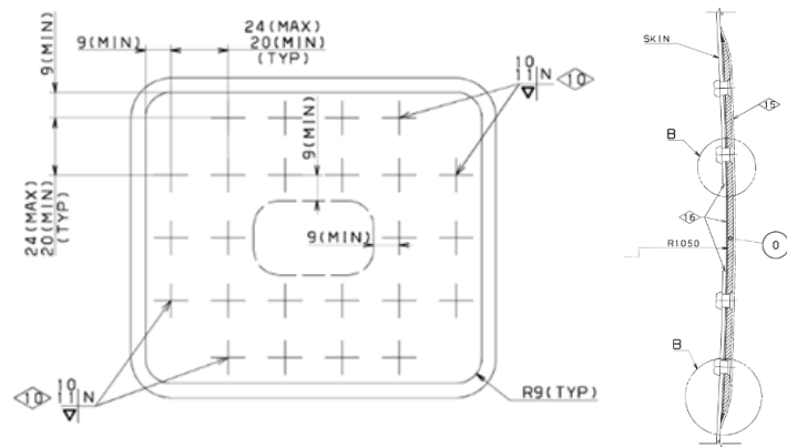
Figure 9. Extract of drawing of a typical bolted repair in a skin panel
