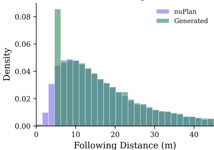
(c) IDM Following Distance
