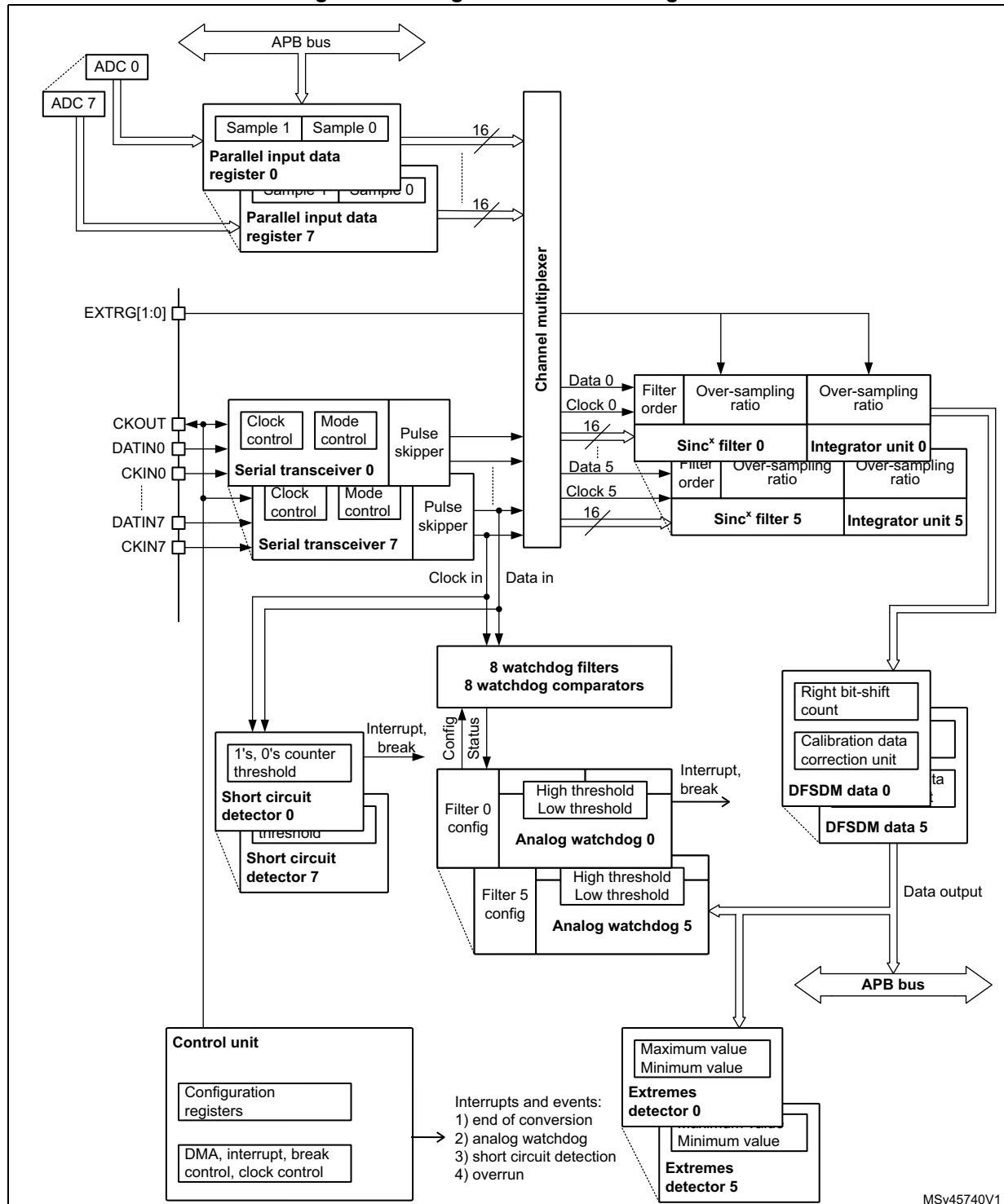
Figure 263. Single DFSDM block diagram
