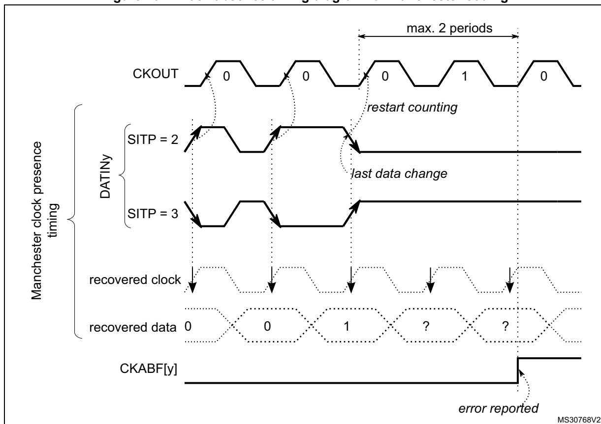
Figure 267. Clock absence timing diagram for Manchester coding
