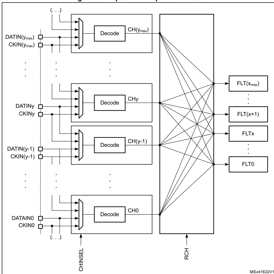
Figure 264. Input channel pins redirection
