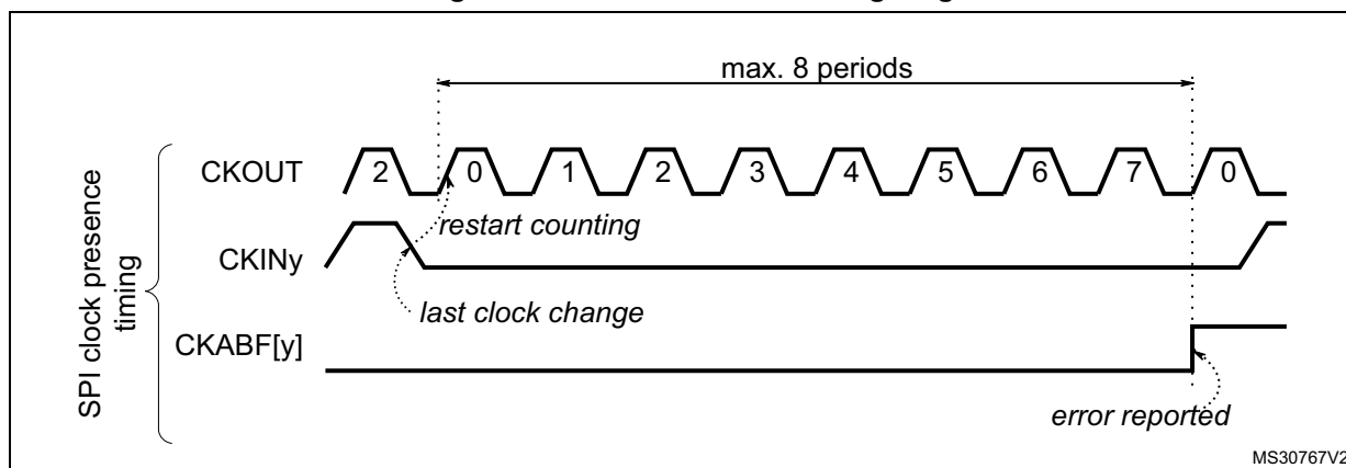
Figure 266. Clock absence timing diagram for SPI
