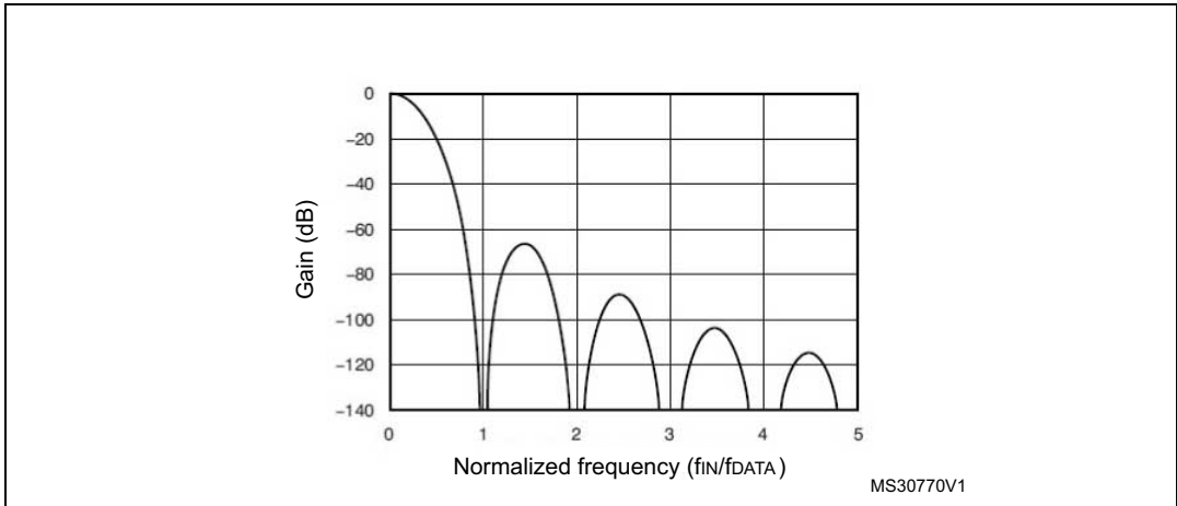
Figure 270. Example: Sinc 3 filter response
