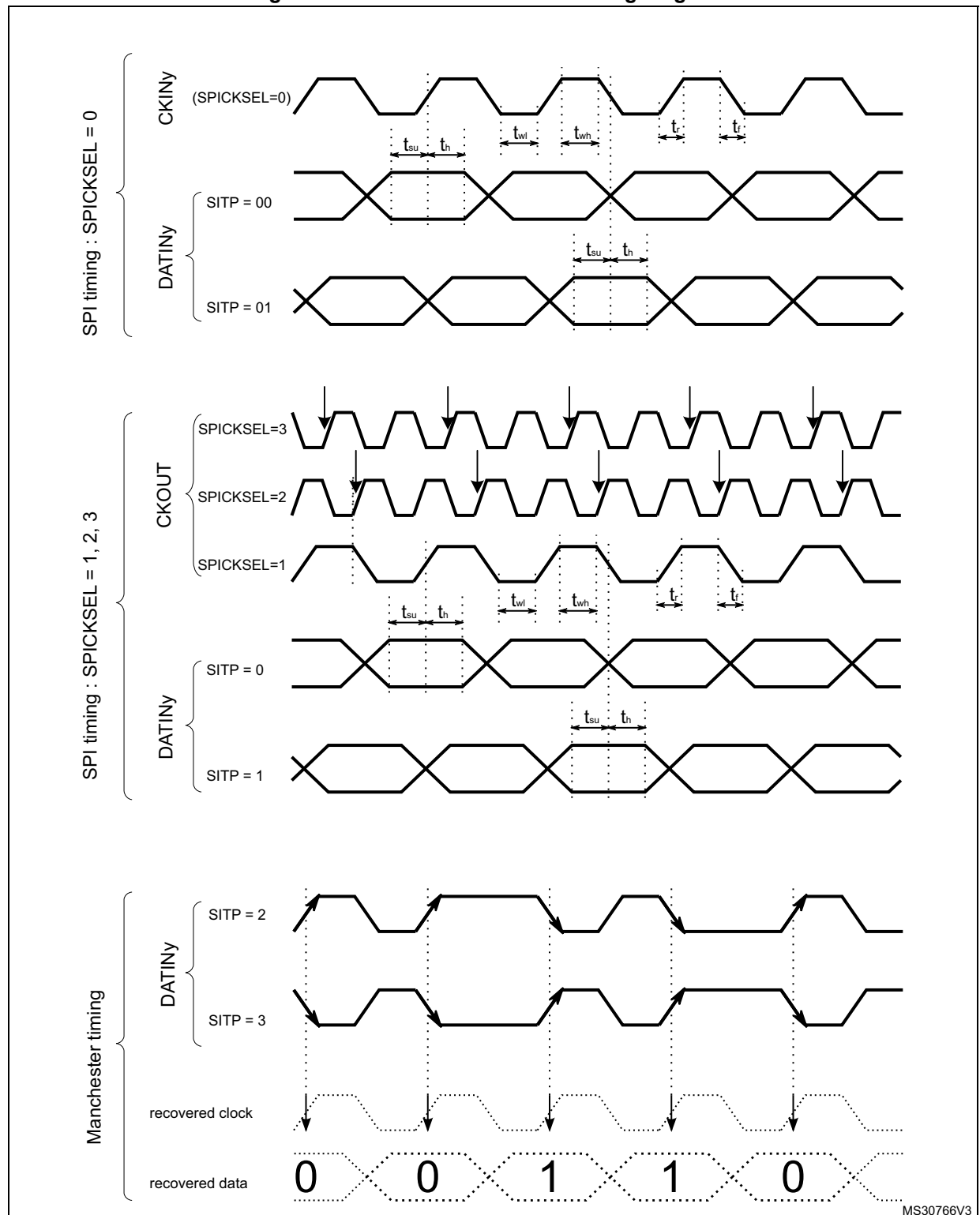
Figure 265. Channel transceiver timing diagrams
