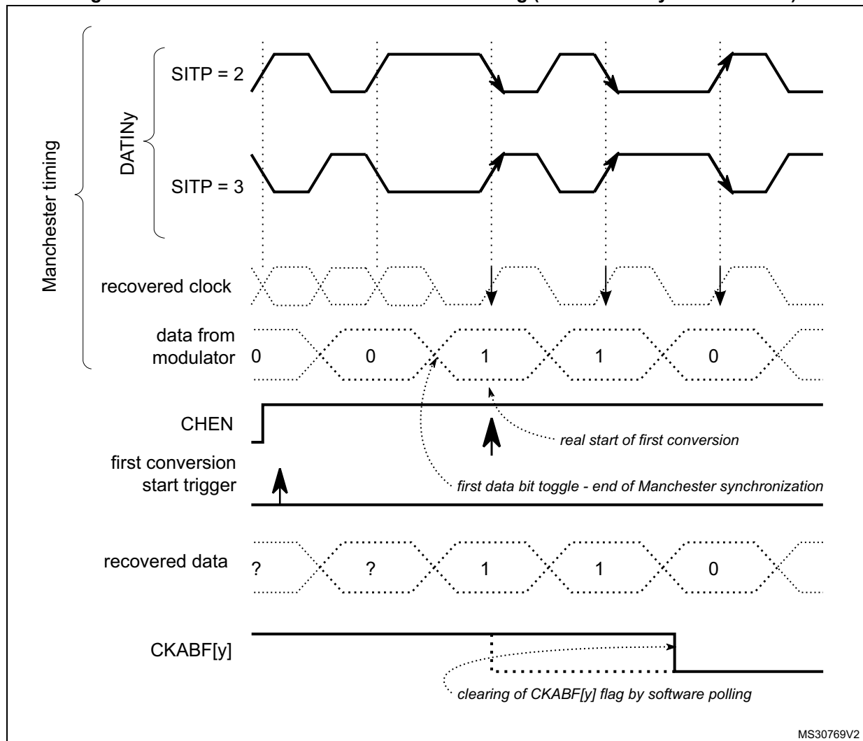
Figure 268. First conversion for Manchester coding (Manchester synchronization)
