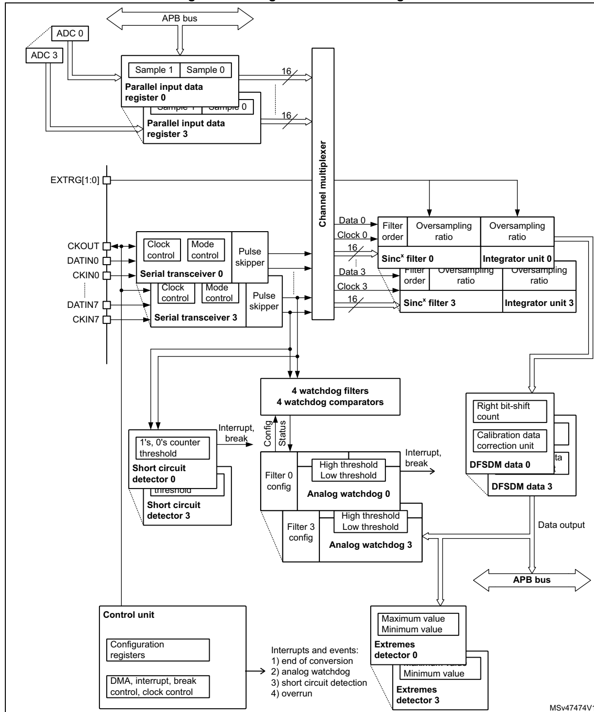
Figure 180. Single DFSDM block diagram
