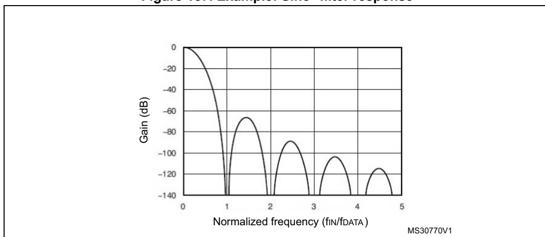
Figure 187. Example: Sinc 3 filter response
