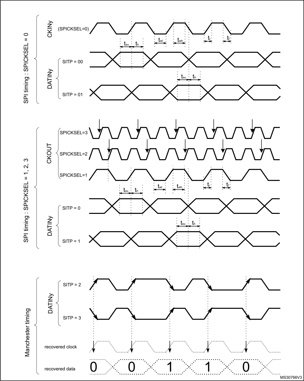
Figure 182. Channel transceiver timing diagrams
