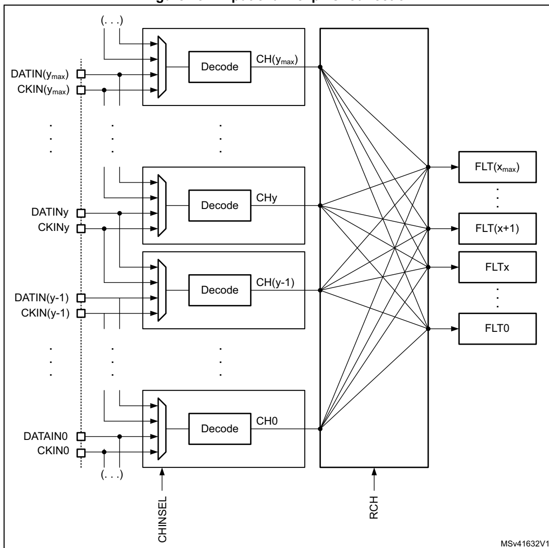
Figure 181. Input channel pins redirection
