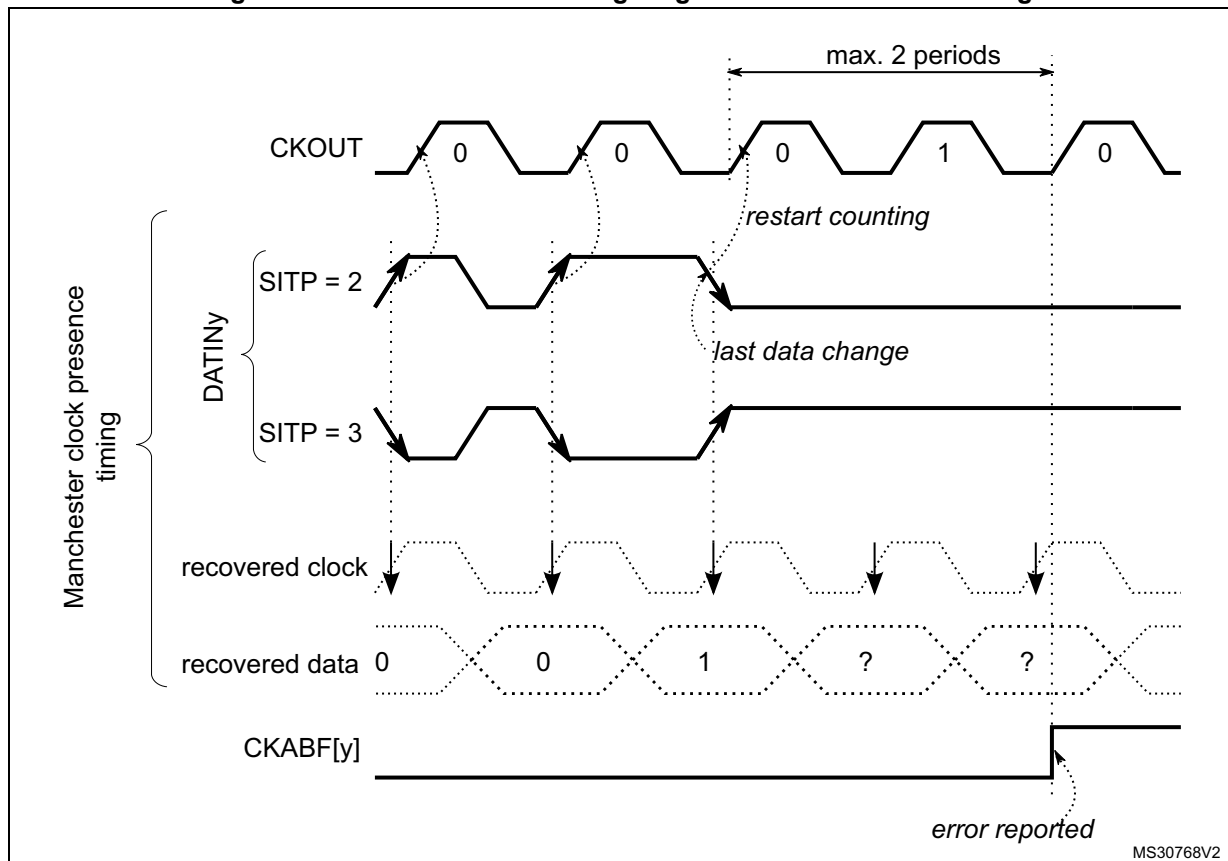
Figure 184. Clock absence timing diagram for Manchester coding
