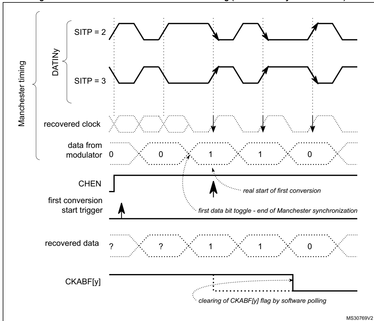
Figure 185. First conversion for Manchester coding (Manchester synchronization)
