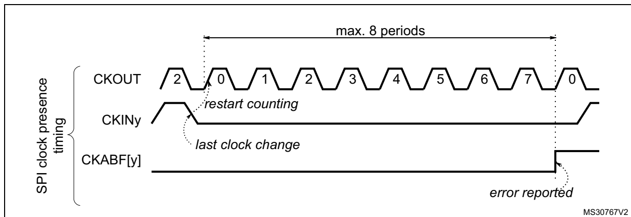
Figure 264. Clock absence timing diagram for SPI
