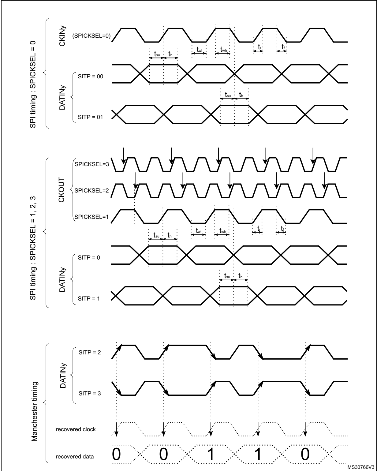
Figure 263. Channel transceiver timing diagrams
