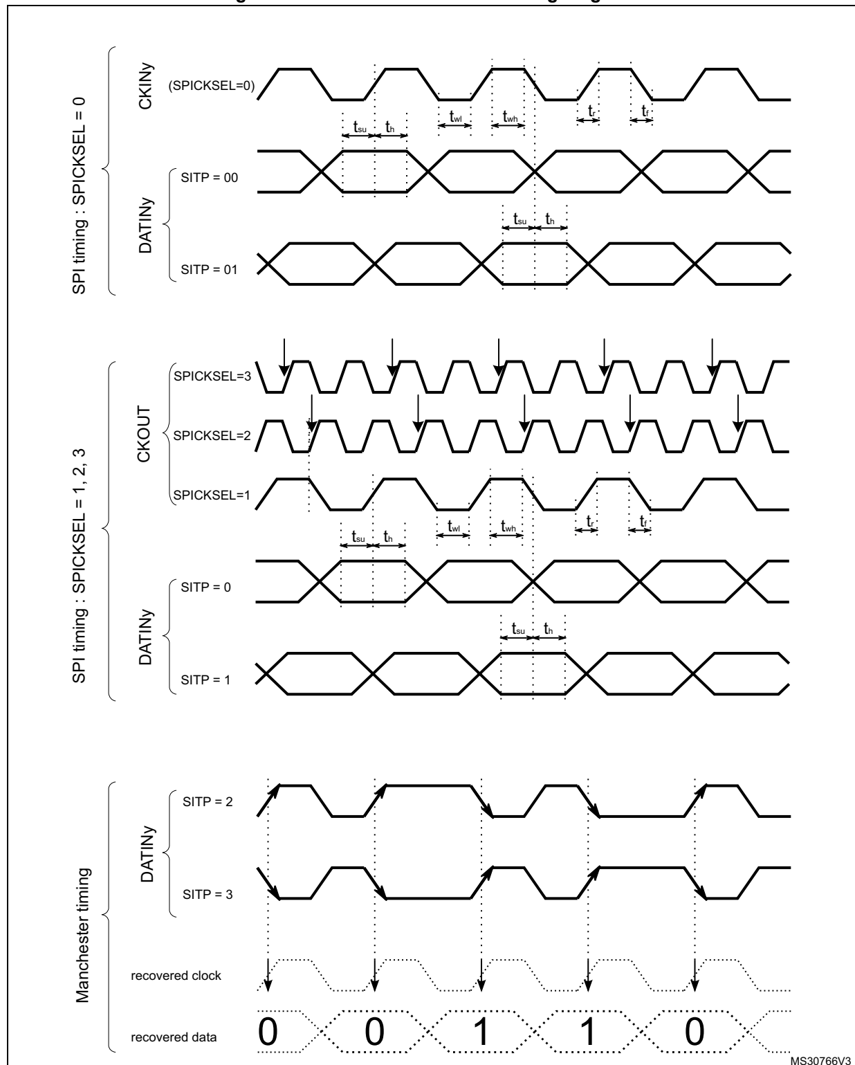
Figure 255. Channel transceiver timing diagrams
