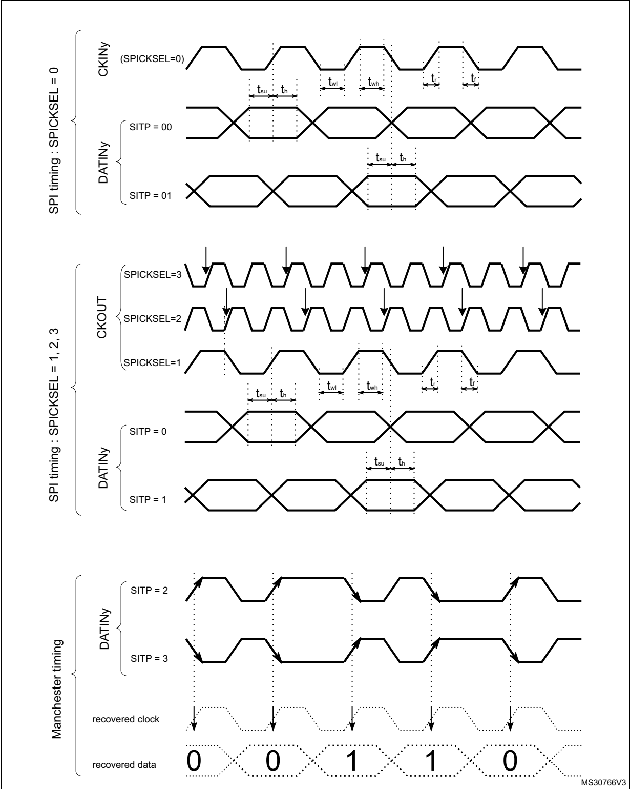
Figure 312. Channel transceiver timing diagrams
