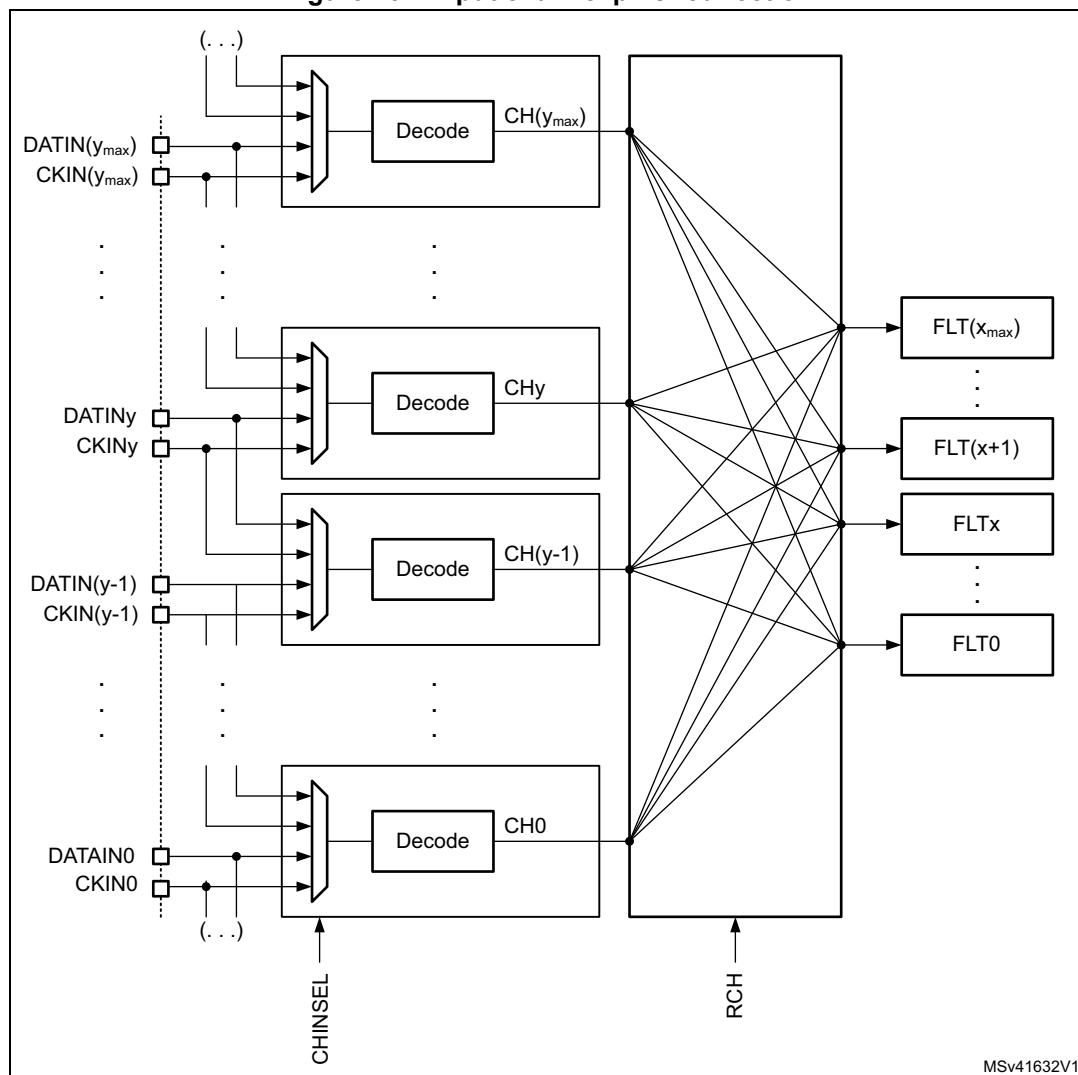
Figure 257. Input channel pins redirection
