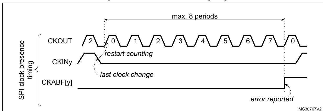
Figure 259. Clock absence timing diagram for SPI
