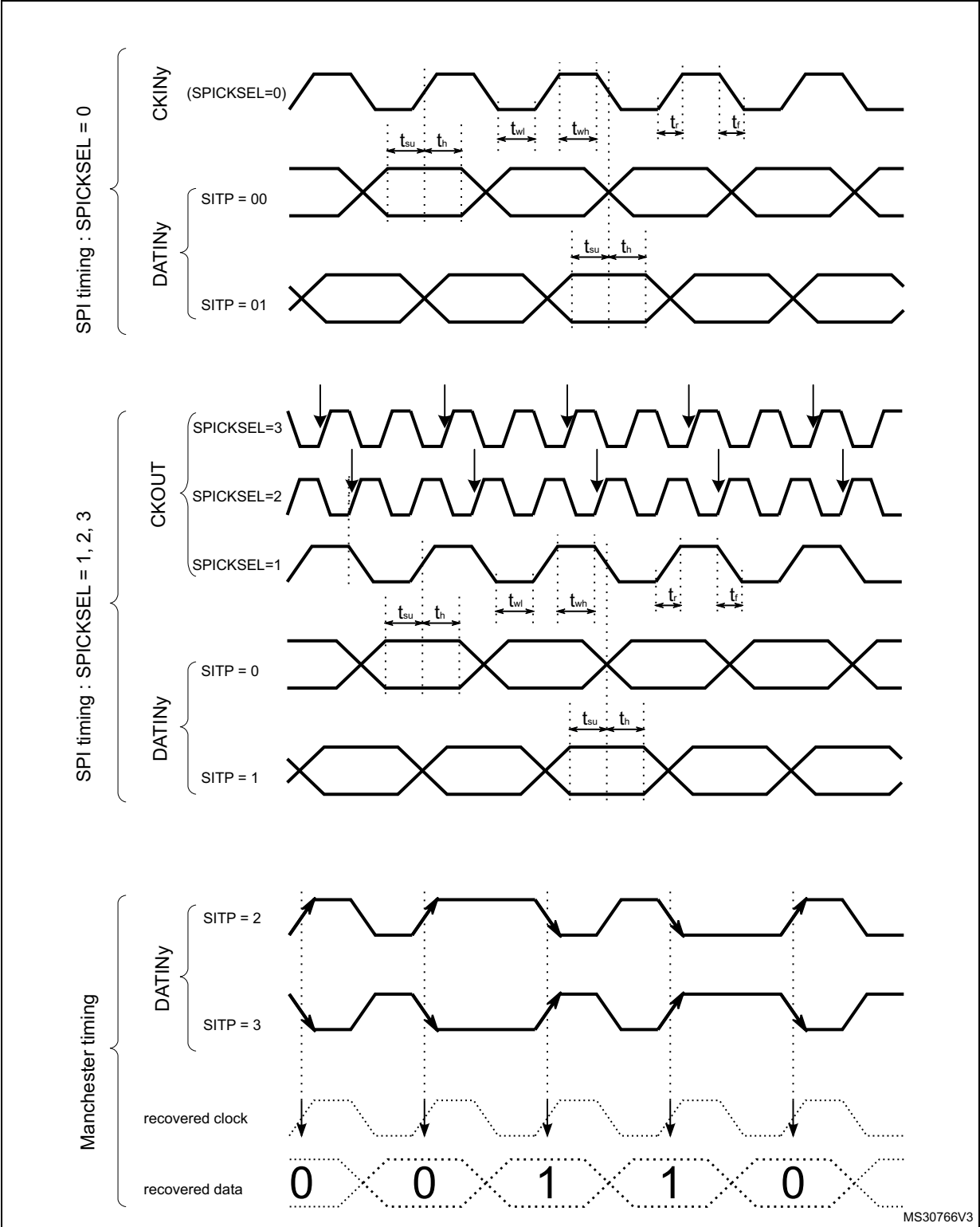
Figure 258. Channel transceiver timing diagrams
