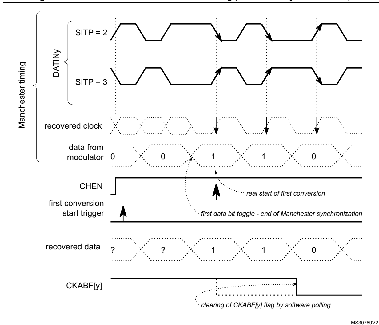
Figure 261. First conversion for Manchester coding (Manchester synchronization)
