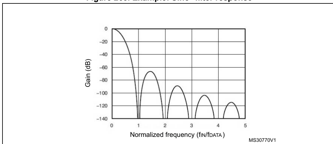
Figure 263. Example: Sinc 3 filter response
