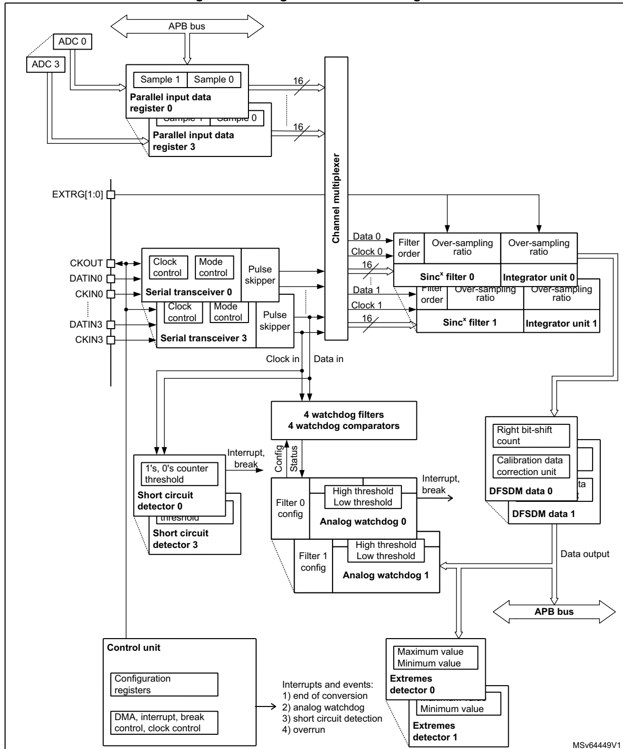
Figure 256. Single DFSDM block diagram
