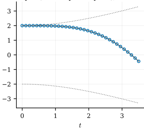
equal (PU exceptional point), \omega = 0.75
