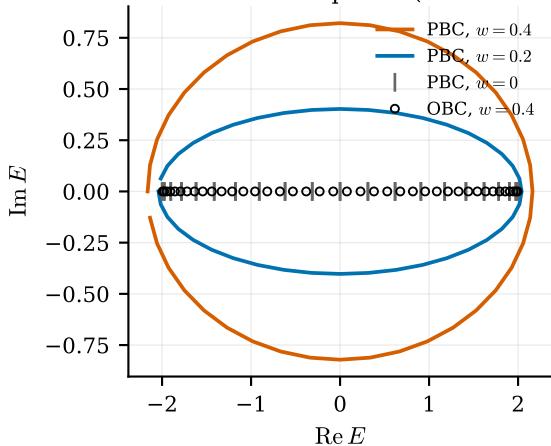
Hatano-Nelson spectra (PBC vs. OBC)
