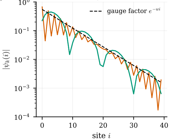
OBC skin modes, w = 0.15
