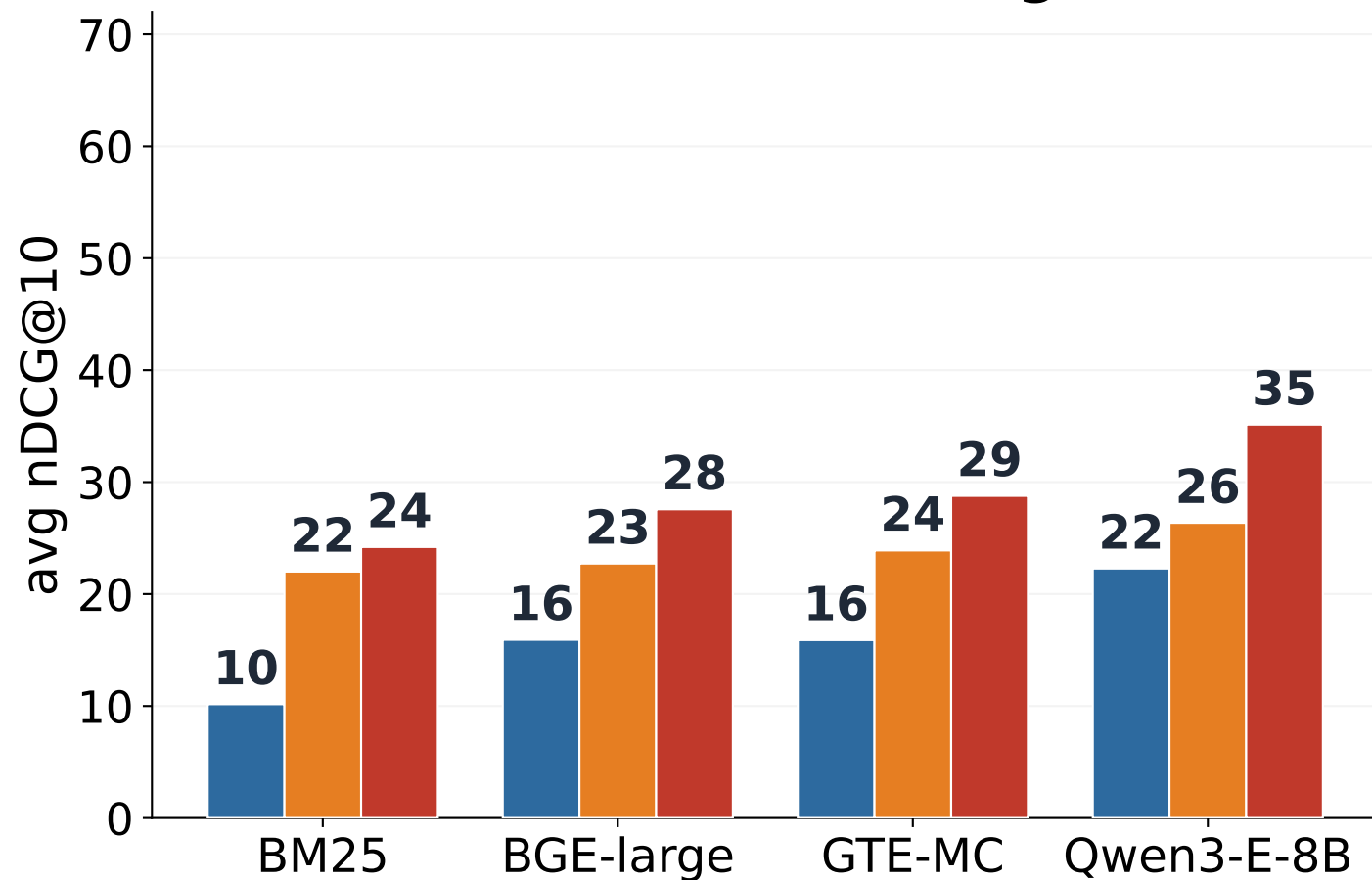
BRIGHT (reasoning)
