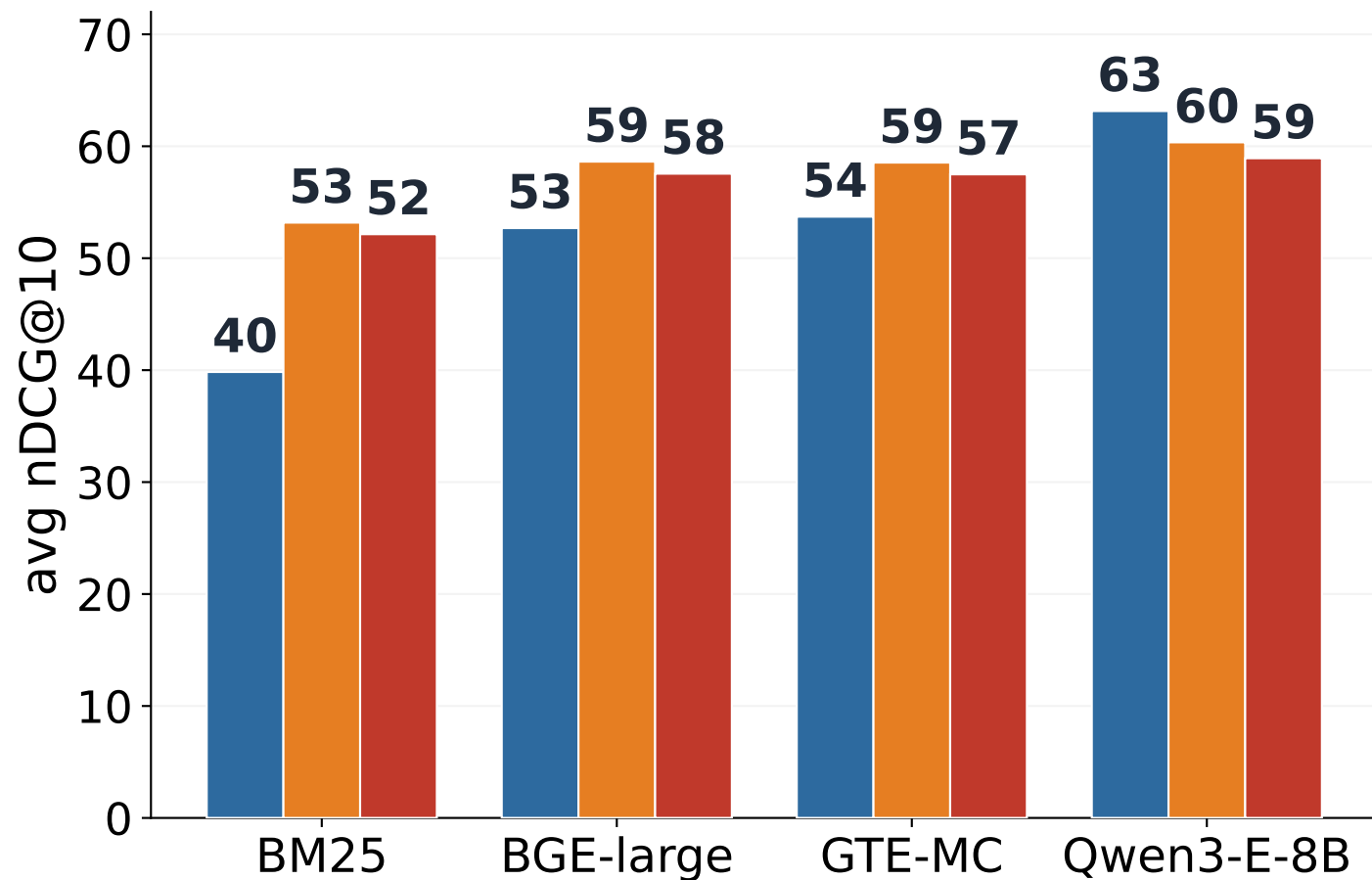
BEIR (semantic)
