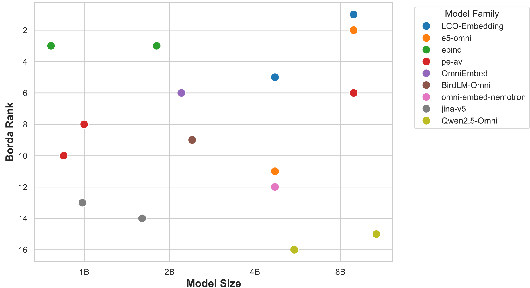
Model Size vs Borda Rank
