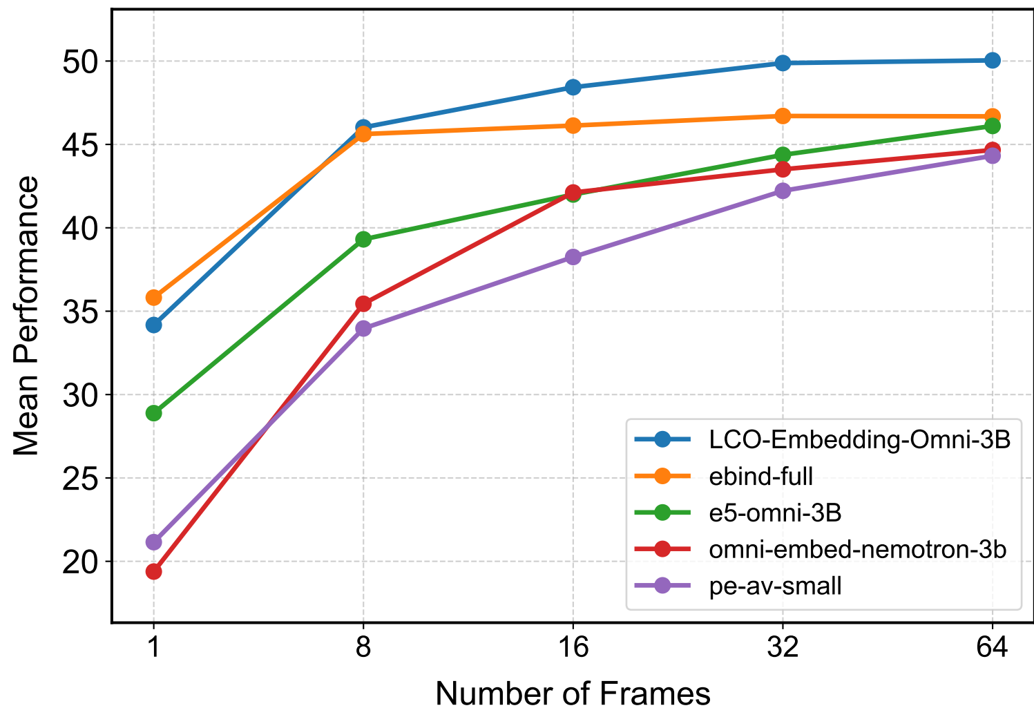
Effect of Frame Count on Model Performance
