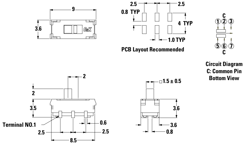
Vertical Mount SMT - J Bend JS202011JCQN DPDT Shown in position B. Available in tap & reel only
